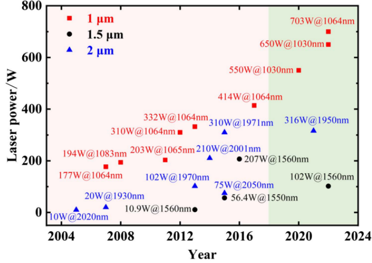
Figure 1: Output power evolution of CW single-frequency amplifiers in all-fiber format operating in 1, 1.5, and 2 \mu\text{m} regions [Li 2023].
