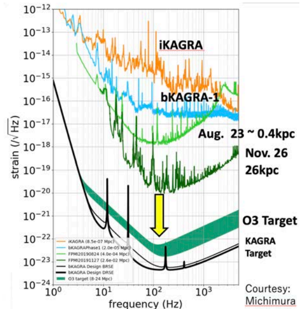
(Above) Comparison of sensitivity curves. Courtesy: Yuta Michimura.
