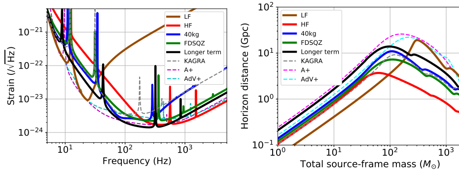
Fig. 2. (Left) Example sensitivity curves for the upgrade of KAGRA using different technologies. LF : Lower input power plan to focus on low frequency. HF : Higher power plan with frequency independent squeezed vacuum to focus on high frequency. 40kg : Sensitivity with increased mass of the test masses from 22.8 kg to 40 kg. FDSQZ : Sensitivity with the injection of frequency dependent squeezed vacuum generated with a 30-m filter cavity. Longer term : Example of longer term upgrade plan combining multiple technologies. Sensitivity curves for A+ 13 and AdV+ 5 are also shown for comparison. (Right) The horizon distance of example KAGRA upgrades for equal-mass, nonspinning binaries. The horizon distance shows the maximum distance at which gravitational waves can be detected with signal-to-noise ratio of more than 8.
