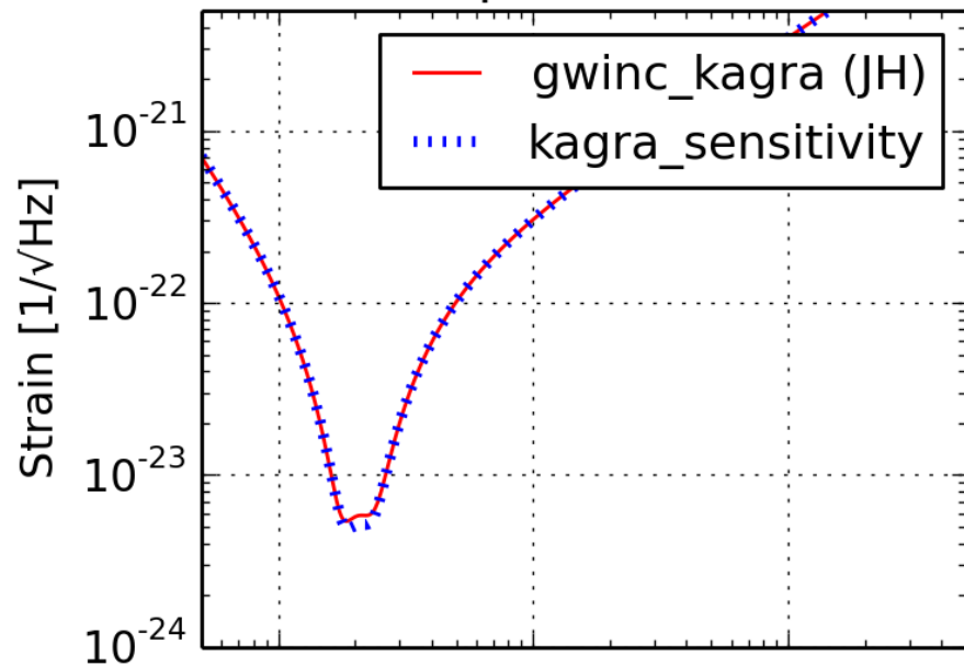
KAGRA+ (LF) [quantum noise]
