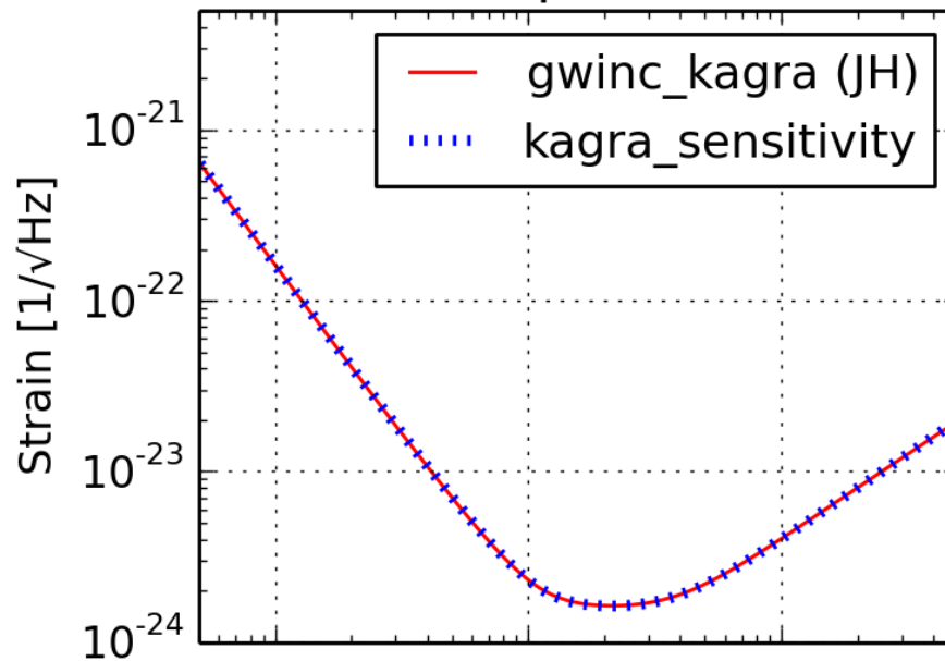
KAGRA+ (FDSQZ) [quantum noise]
