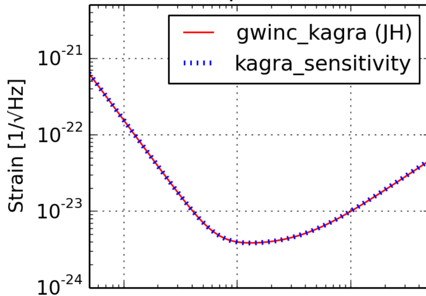
bKAGRA (BRSE) [quantum noise]
