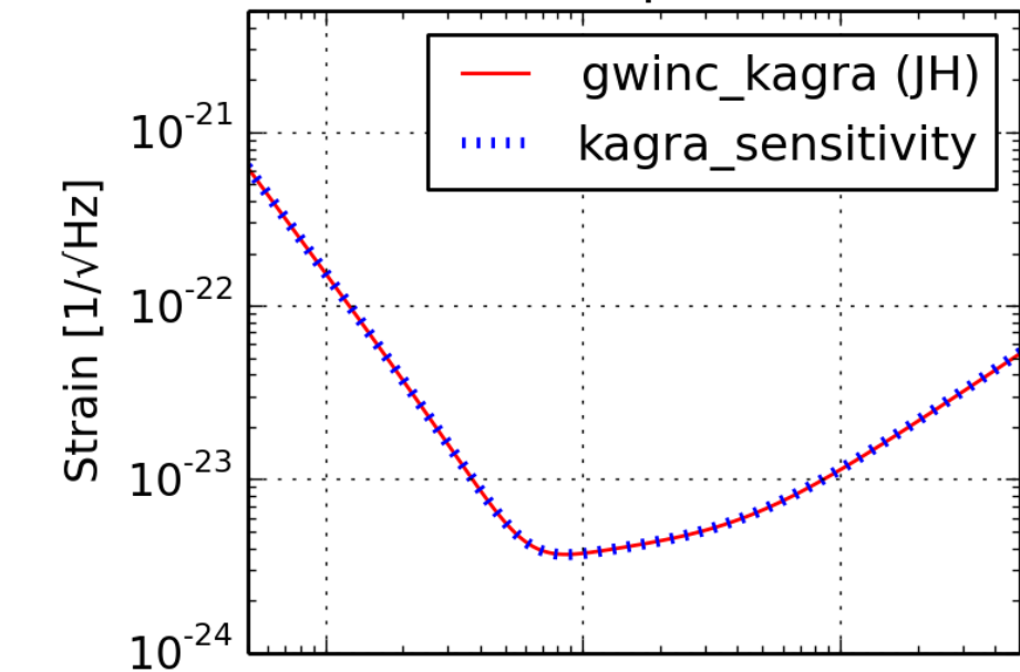
bKAGRA (BRSEhomo) [quantum noise]
