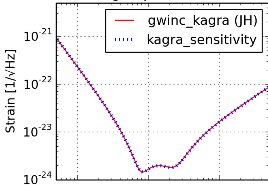
KAGRA+ (40kg) [quantum noise]
