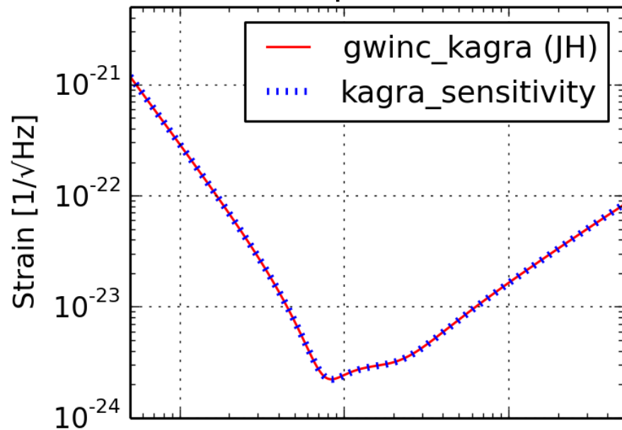
bKAGRA (DRSE) [quantum noise]
