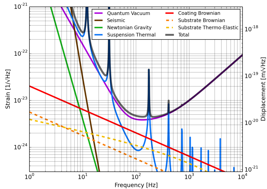
bKAGRA (BRSE)
