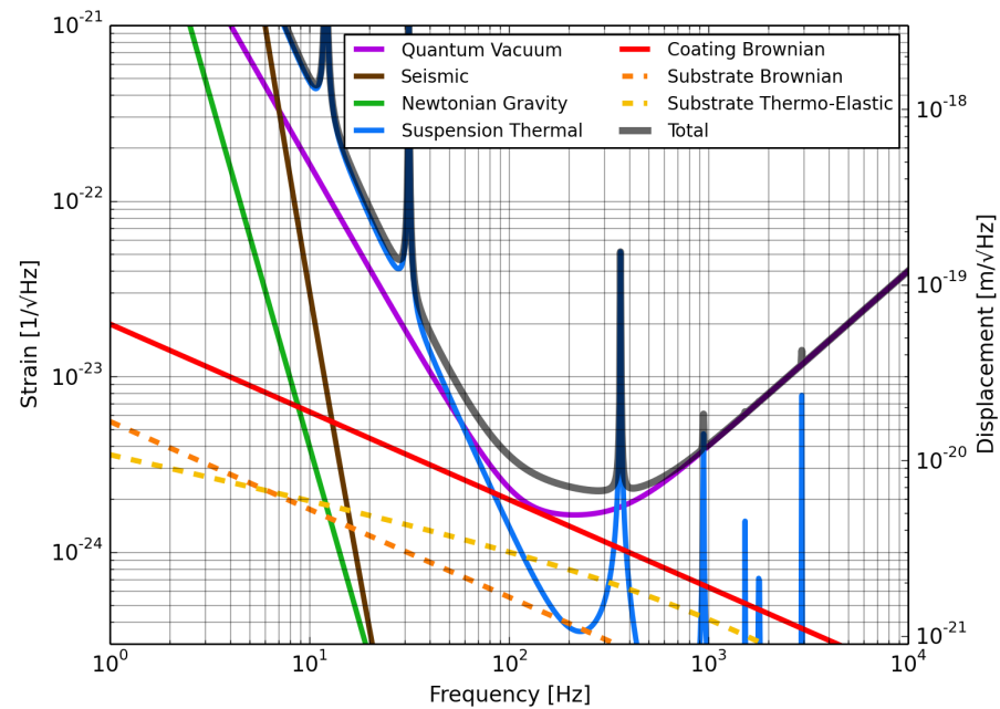
KAGRA+ (FDSQZ)
