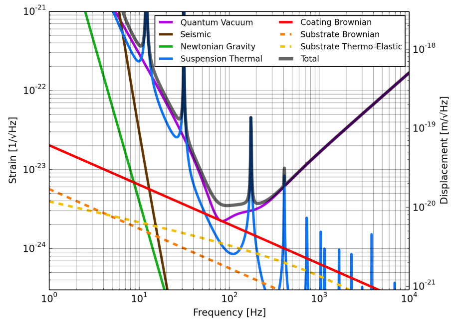
bKAGRA (DRSE)
