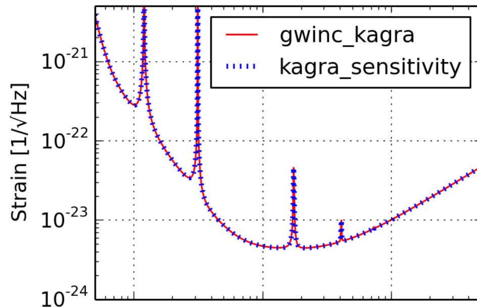
bKAGRA (BRSE)
