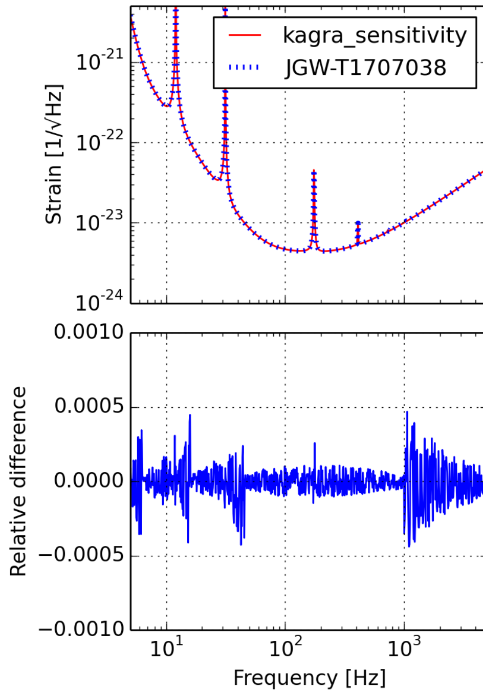
bKAGRA (BRSE)
