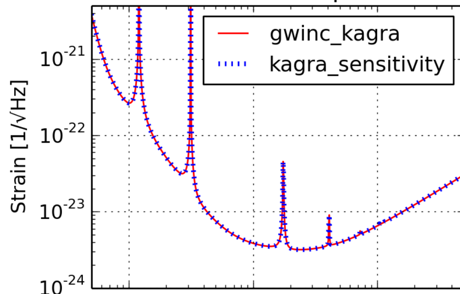
bKAGRA (BRSEsqz)
