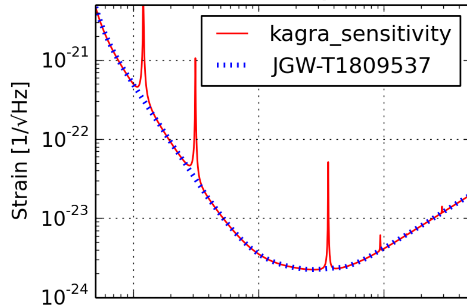
KAGRA+ (FDSQZ)
