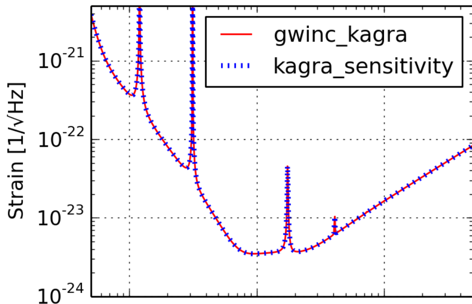
bKAGRA (DRSE)
