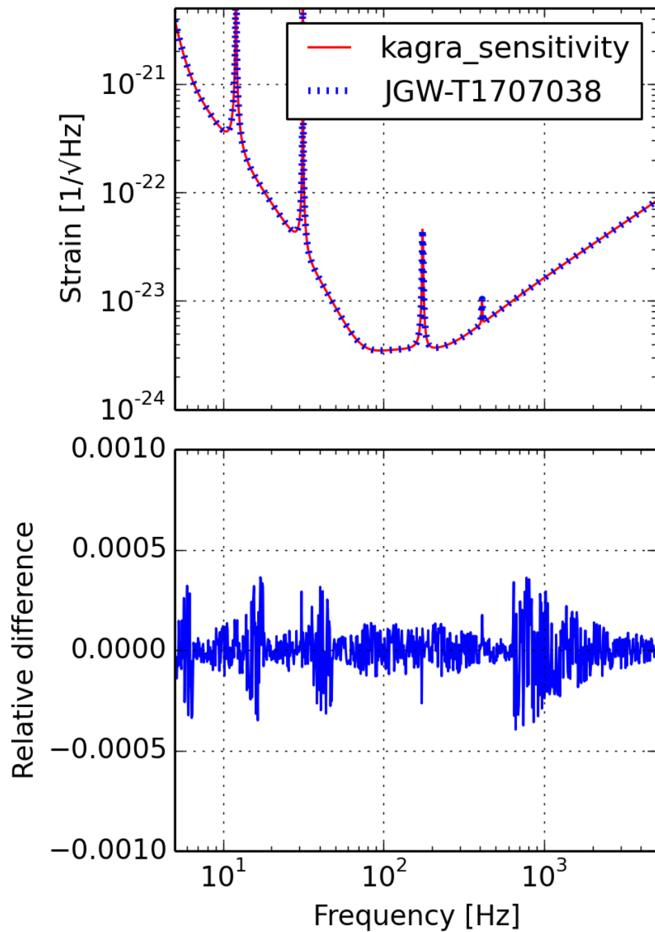
bKAGRA (DRSE)
