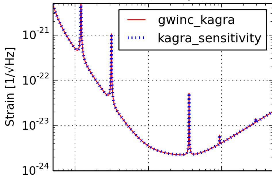
KAGRA+ (FDSQZ)
