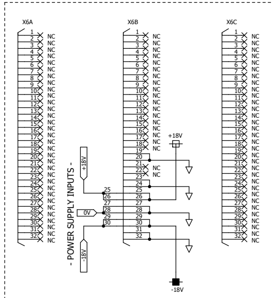
VME top connector
