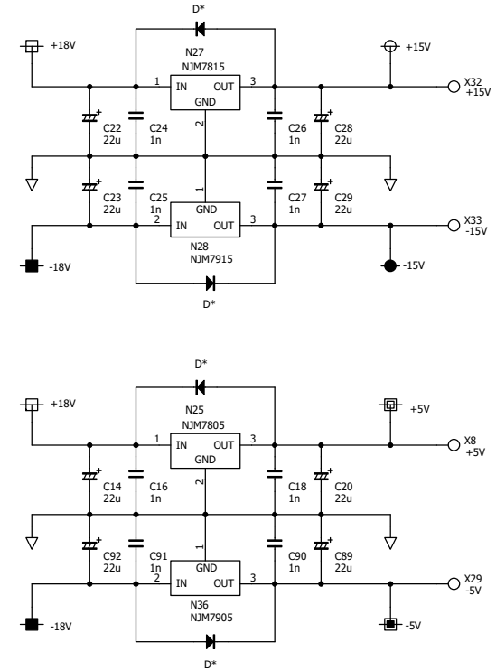
Linear regulator
