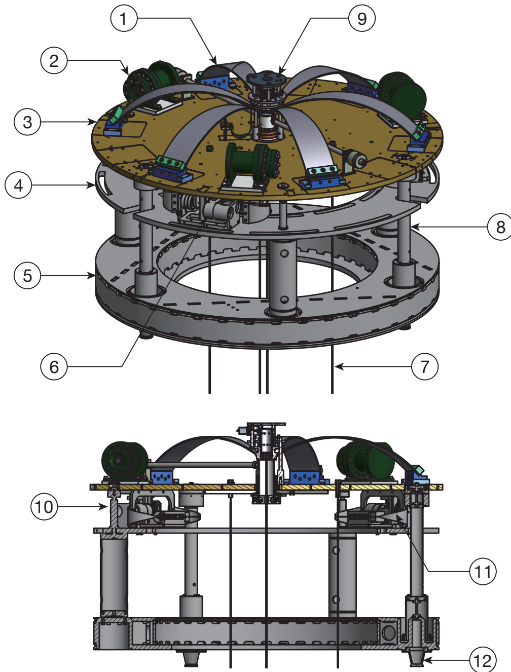
Fig. 3.9. An overview of the pre-isolator ( top ) and its cross-section view ( bottom ). The numbered components are the 1) cantilever blade, 2) geophone capsulated in a vacuum canister, 3) table of the top stage, 4) reference frame rigidly connected to the base ring, 5) base ring, 6) unit of the LVDT and the coil-magnet actuator, 7) suspension wires, 8) IP leg, 9) keystone and the surrounding structure of the top filter, 10) lock pillar for the top stage, 11) motorized blade spring for static position control of the top stage and 12) cup of the cone bellows.
