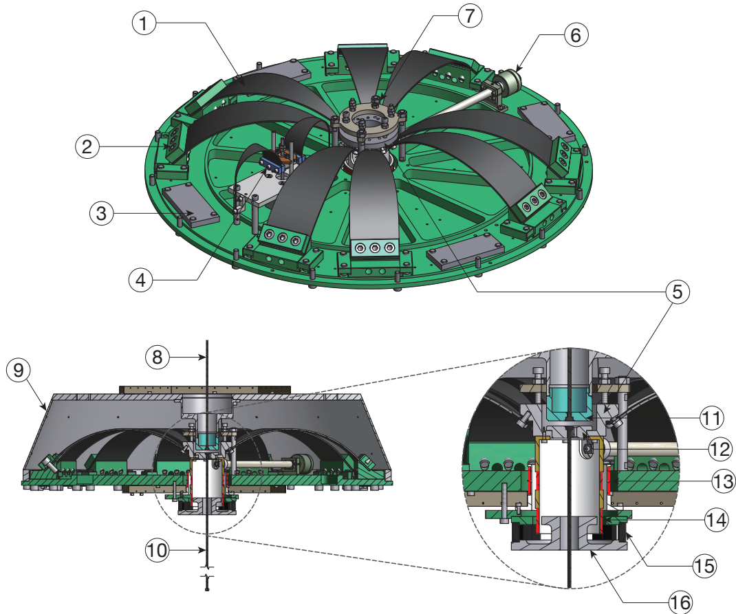
Fig. 3.11. An overview of the standard GAS filter without the cap ( top ) and its cross-section view with the cap ( bottom ). The numbered components are the 1) cantilever blade, 2) blade clamp, 3) ballast mass, 4) fishing rod, 5) keystone, 6) magic wand, 7) lock screws and nuts, 8) upper suspension wire, 9) filter cap, 10) lower suspension wire, 11) wire receptacle for the upper wire, 12) wire receptacle for the lower wire, 13) coils for LVDT displacement sensor, 14) actuator coil, 15) magnets and 16) iron yoke.
