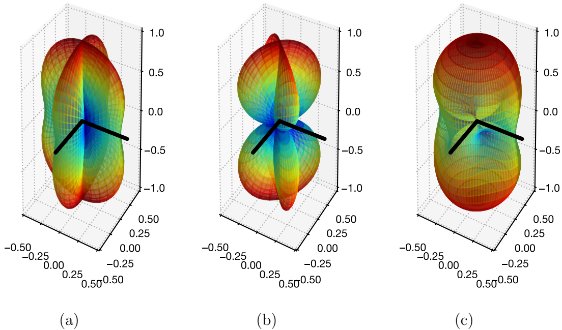
Fig. 1.10. Antenna patterns of the interferometric gravitational wave telescope to the (a) + -mode, (b) \times -mode and (c) squared average of both two modes. The baselines of the interferometer is also illustrated as the L-shaped black lines.
