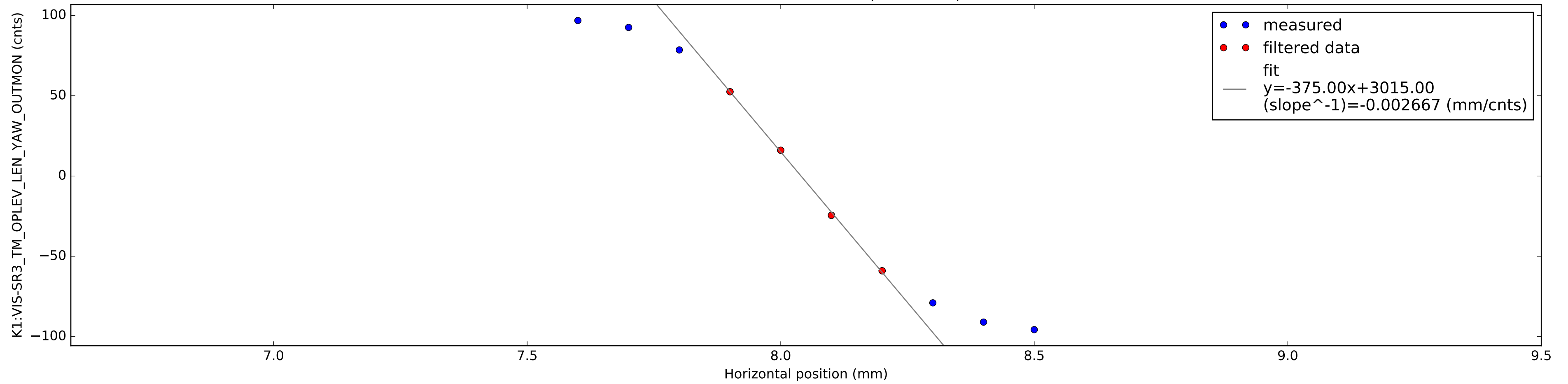
SR3 OPLEV Len Calibration (Horizontal)
