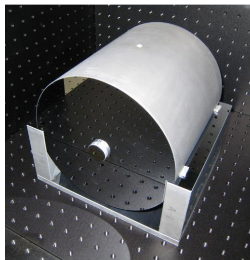
Cryogenic silicon cavity
