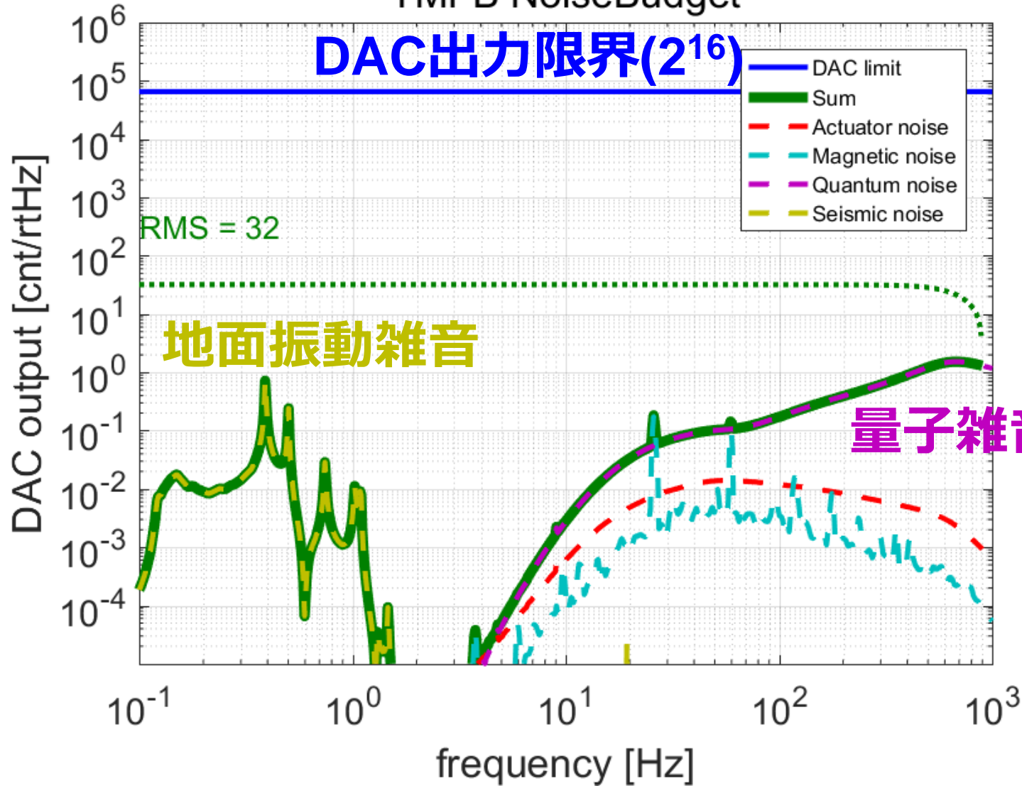
TMFB NoiseBudget
