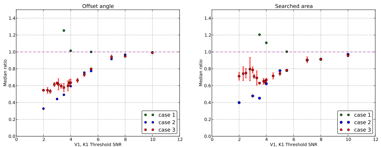
Figure 11.1: Offset angle ( Left ), searched area ( Right ) with 4 detector hierarchical search. In case 3 investigation, calculation is repeated for two times, using different set of random numbers.
