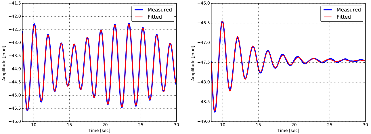
Figure 5.32: A example of measured decay signals. Left shows the signal from passive system of mode #3 and #5. Right describes the signal of mode #3 with active control. These signals are measured by the virtual pitch sensor at IM-OSEM. The measured frequencies and decay time without control were 0.46 Hz, 70 sec for mode #3 and 0.52 Hz, 91 sec for mode #5. Those with control were 0.47 Hz, 4 sec.
