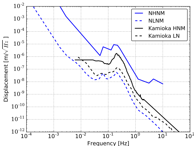
Figure 2.1: The worldwide seismic noise from J. Peterson’s study (blue) and seismic motion measured at Kamioka underground (black). The blue and dashed-blue line show the new high-noise model (NHNM) and the new low-noise model (NLNM) respectively. The black and dashed-black lines denote the seismic motion in the environment underground at Kamioka mine. The Kamioka HNM (high noise model) shows modeled spectra based on measurement of high-noise seismic motion, and Kamioka LN (low noise) shows a measurement when the seismic noise was low.
