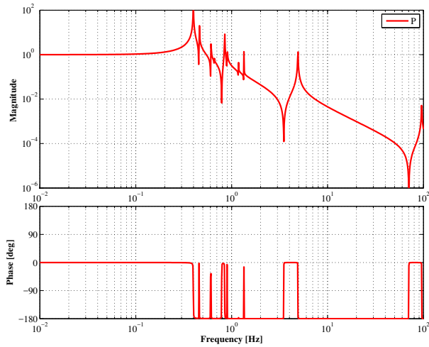
Figure 6.22: IM-OSEM (Pitch)
