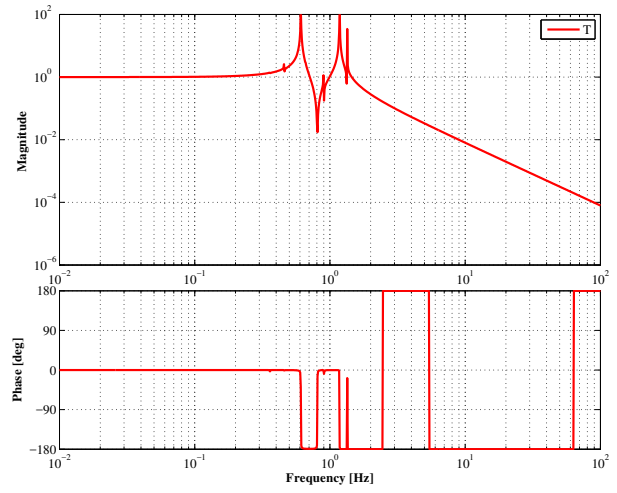
Figure 6.19: IM-OSEM (Transversal)
