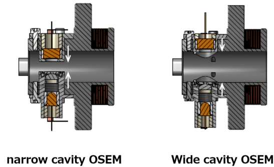
Figure 6.6: Overview of the OSEM in iKAGRA-PR3 SAS ( left , ‘narrow cavity OSEM’) and that in the type-Bp SAS ( right , ‘wide cavity OSEM’). The gap is widened by 10 mm and the gap of the new system is 15 mm.
