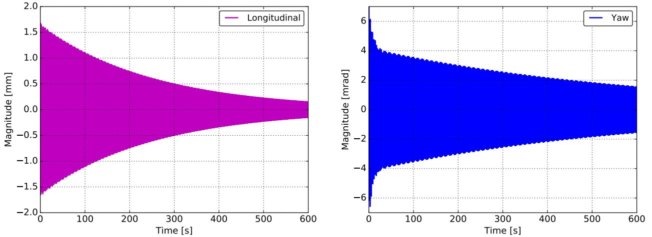
Figure 6.35: Expected 1/e decay time of longitudinal ( left ) and yaw ( right ) motion of the test mass with the active control in the calm-down phase (without the control loops for the test mass).
