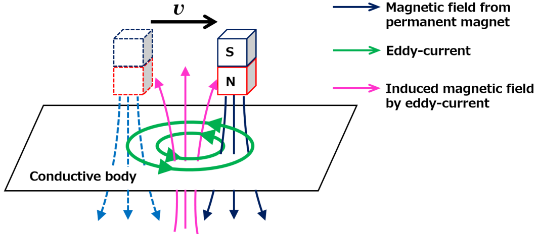
Figure 2.8: Working mechanism of an eddy-current damping system.
