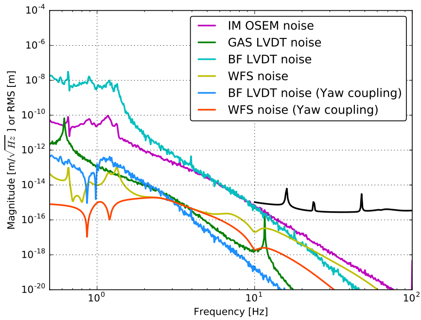
Figure 6.45: Control noise coupling to longitudinal displacement of the TM in the observation phase. This performance is obtained with IM-OSEM loops.
