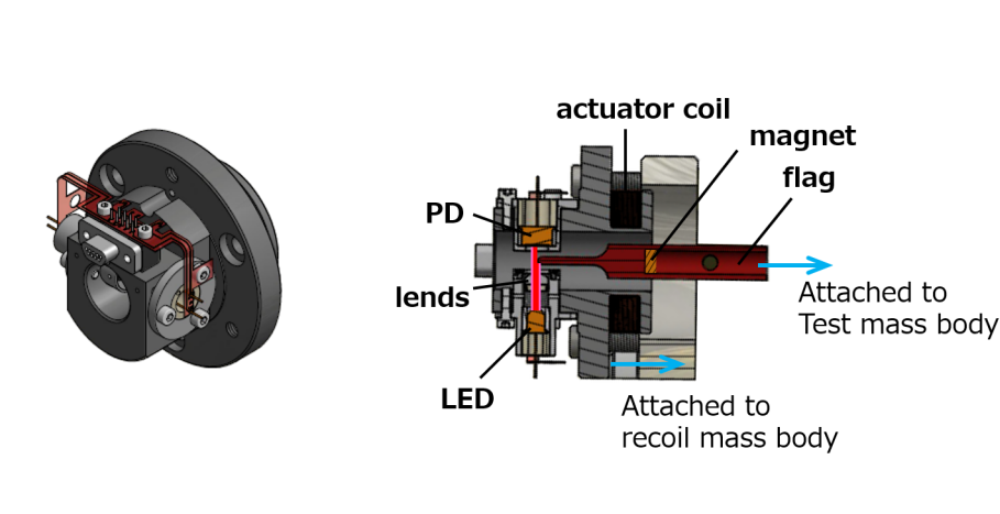
Figure 5.12: Overview view of OSEM unit used in iKAGRA ( left ) and its cross section ( right ). Gap between its PD and the LED was 5 mm.
