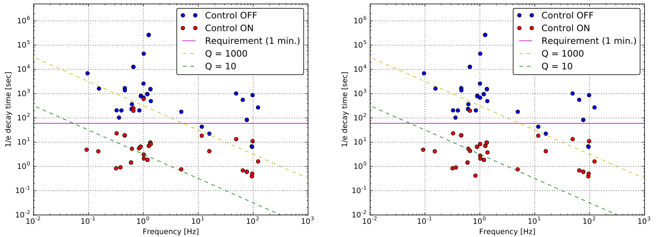
Figure 6.33: Expected 1/e decay time for each mechanical resonances in the type-Bp SAS with and without active control. Left plot shows the performance when the active control with optical sensors are not available, while right plot describes that when the controls with the optical sensors are included.
