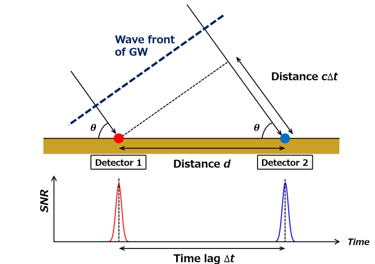
Figure 7.1: Principle of triangulation.
