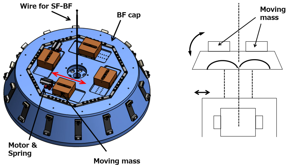
Figure 6.3: Overview of tilt aligning system at BF ( left ). Right figure shows the behavior of the BF, IR, and IM. Moving mass on the BF cap adjusts the gap between the IR and IM.
