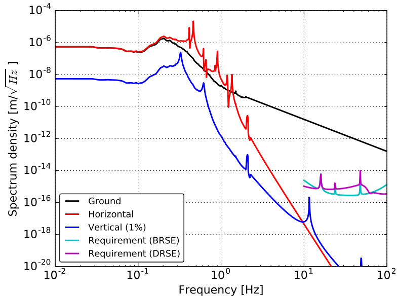
Figure 3.9: Predicted seismic isolation performance of the type-Bp SAS compared with the requirements and the seismic vibration. It assumes 1 % vertical-horizontal coupling.
