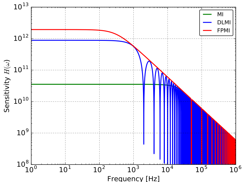
Figure 1.4: Amplitudes of the frequency responses H_{\text{MI}} , H_{\text{DLMI}} and H_{\text{FPMI}} with 3 km arm length. The value of N for Delay-line Michelson interferometer (DLMI) is set at 50. The finesse \mathcal{F} is set at 80 for Fabry-Perot Michelson interferometer (FPMI). Here the wavelength of the laser is \lambda = 1064 nm. MI denotes Michelson interferometer.
