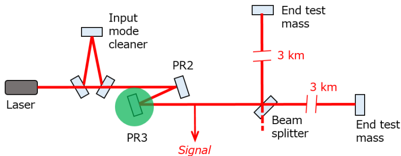
Figure 5.1: Optical configuration of the iKAGRA interferometer. The iKAGRA-PR3 SAS was installed at green circled area, which is situated on the central room of the KAGRA tunnel.
