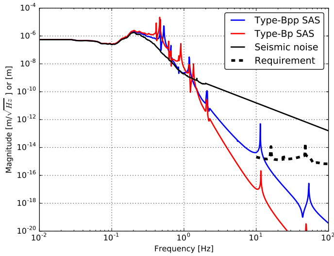
Figure 5.38: The simulated vibration isolation performances of the iKAGRA-PR3 SAS (blue), and that of the type-Bp SAS (red) without active controls. The ground displacement (black) and the requirement (dashed-black) are also shown in this plot. By adding one more GAS filter into the iKAGRA-PR3 SAS, the system is able to meet its requirement.
