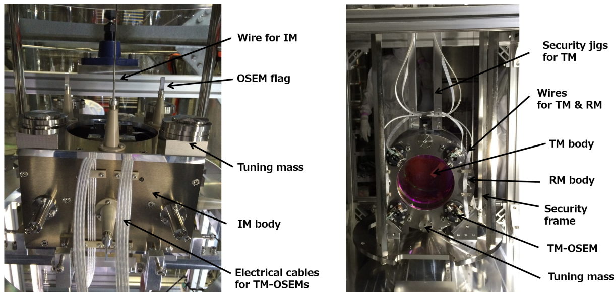
Figure 5.5: Overview of the assembled payload. Left figure shows the assembled IM, while the right depicts the assembled TM and RM.
