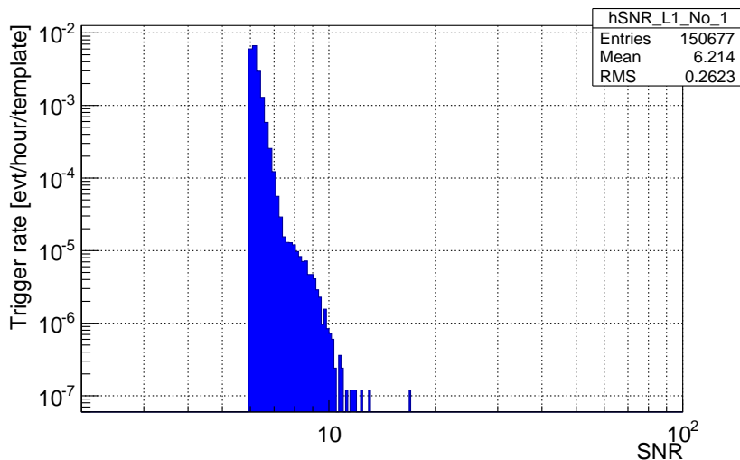
Figure 9.4: An example of the background SNR distribution measured at L1 detector in O1 run.
