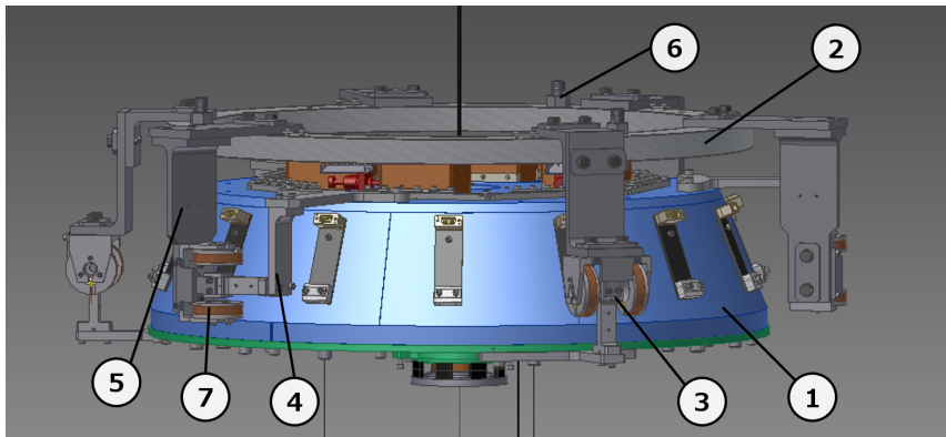
Figure 3.7: Overview of the bottom filter damping system. 1) The body of the bottom GAS filter, 2) the recoil mass for the bottom GAS filter, 3) the BF-LVDT and coil-magnet actuator unit, 4) the magnet holder of BF-LDVDT unit, 5) the coil holder of BF-LDVDT unit, 6) the hook for the suspension wire connects to beneath of the standard GAS filter, 7) the BF-LVDT coil.
