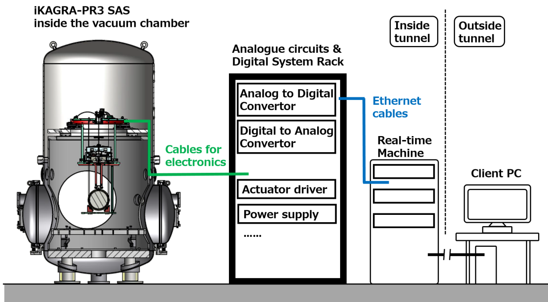
Figure 5.2: Overview of the experimental setup for the iKAGRA-PR3 SAS performance test.
