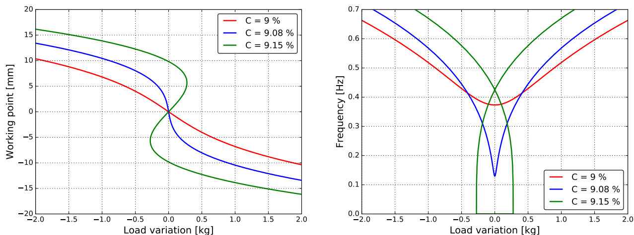
Figure 2.11: Behavior of the working point of the keystone ( left ) and its resonant frequency ( right ) with various compression of the GAS blade, as a function of tip load of the suspended payload, and which are obtained through the model. In the right plot, it is assumed m_0 = 200 kg.
