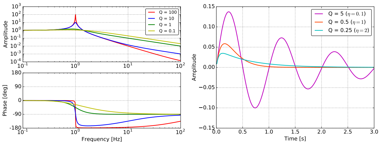
Figure 2.7: The amplitude and the phase of H(\omega) ( left ) and the response of a damped mechanical oscillator to an impulsive force injected to the suspended mass ( right ), with various Q factors (viscous damping factors) .
