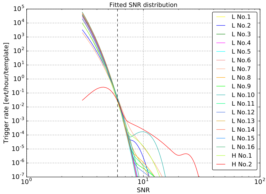
Figure 9.5: Examples of fitted background SNR distribution at H1 and L1 detector in O1 run.
