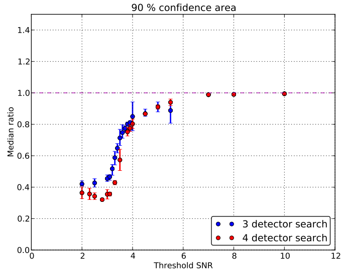
Figure 11.8: Comparison of 90 % confidence area between 3 detector hierarchical search and 4 detector search. At below SNR 4, the area is further reduced due to the contribution of quadruple triggers than 3 detector hierarchical network.
