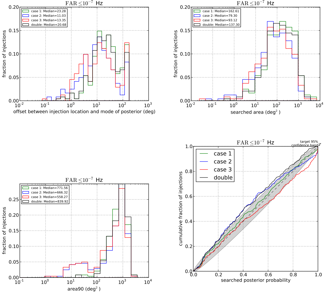
Figure 10.3: Offset angle ( upper left ), searched area ( upper right ), cumulative 90 % confidence area ( lower left ), P-P plot ( lower right ). The green, blue, red, black curves correspond to case 1, case 2, case 3 with 3-detector search with HLV, and 2-detector search with HL, respectively.
