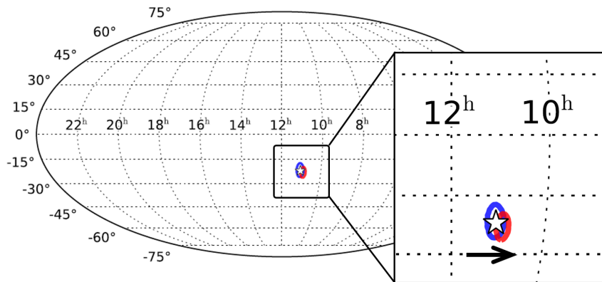
Figure 8.3: Effect of noise curve on its prediction. Blue circled map is generated with using only timing error based on noise curve. Red map is from both of the timing error based on the noise curve and arrival timing.
