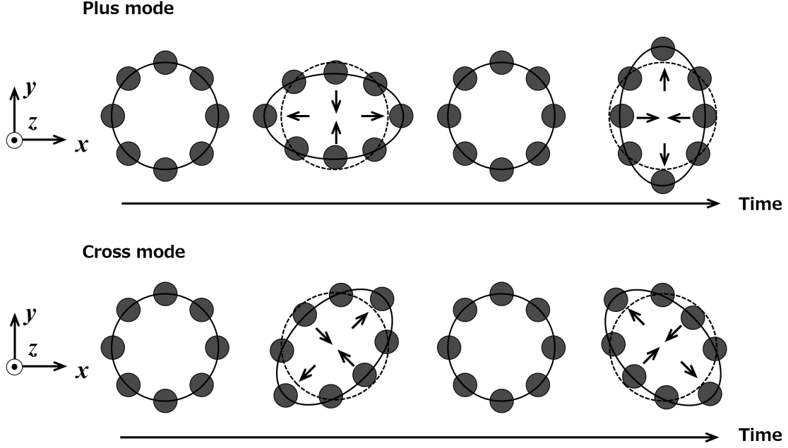
Figure 1.1: Polarizations of a gravitational wave. If a gravitational wave incidents into +z axis, the positions of free particles arrayed in circle are changed as shown in this figure. Black points denote free particles.
