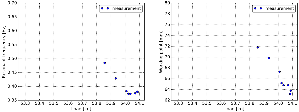
Figure 5.4: Measured bottom GAS filter response. Left plot shows the load dependence of the resonant frequency and right plot shows the load dependence of the working point.
