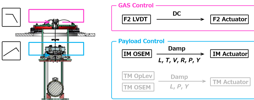
Figure 5.29: Control loops of the iKAGRA-PR3 SAS in the calm-down phase.
