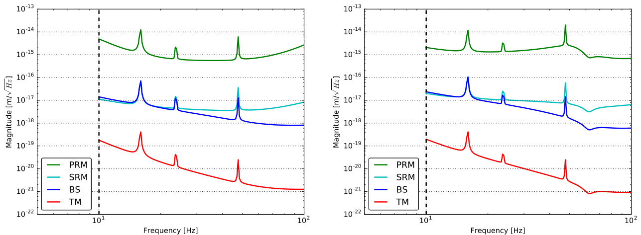
Figure 3.1: Displacement requirement in BRSE detection mode ( left ) and DRSE detection mode ( right ). PRM, SRM, BS, and TM denote power recycling mirror, signal recycling mirror, beam splitter, and test mass respectively.
