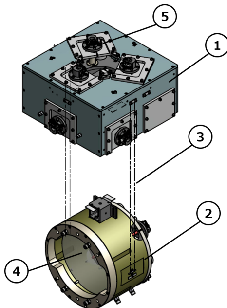
Figure 3.8: Overview of the payload of the type-Bp SAS. 1) The body of the intermediate recoil mass, 2) the recoil mass for the test mass, 3) the wires to suspend the recoil mass of the test mass, 4) the test mass, 5) the OSEM unit. The intermediate mass is covered by the intermediate recoil mass in this figure.
