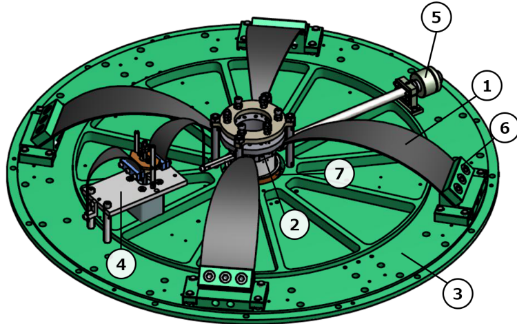
Figure 3.5: Overview of the standard GAS filter. 1) The cantilever blade, 2) the keystone, 3) the baseplate, 4) the motorized spring for initial positioning of the keystone, 5) the magic-wand for compensating CoP effect, 6) the base clamp, 7) the LVDT to monitor the displacement of the keystone.
