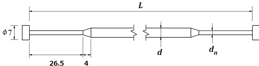
Figure 3.6: Designed suspension wire.
