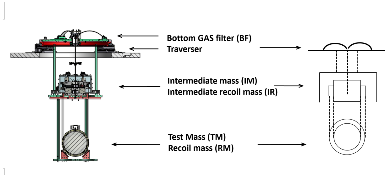
Figure 5.3: Cross section of the iKAGRA-PR3 SAS components.
