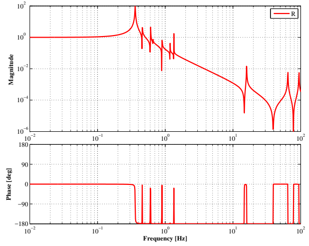
Figure 6.21: IM-OSEM (Roll)
