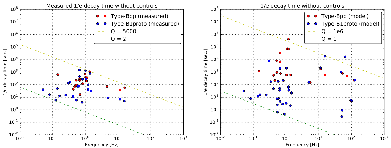
Figure 5.37: Decay time constants of the mechanical resonances without the active control. Left plot shows the measured results and right plot shows the simulated ones.
