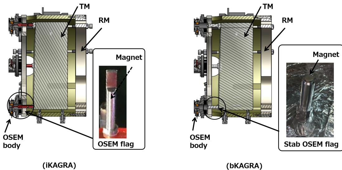
Figure 6.8: Difference of the OSEM system between the iKAGRA-PR3 SAS ( left ) and the type-Bp SAS ( right ).
