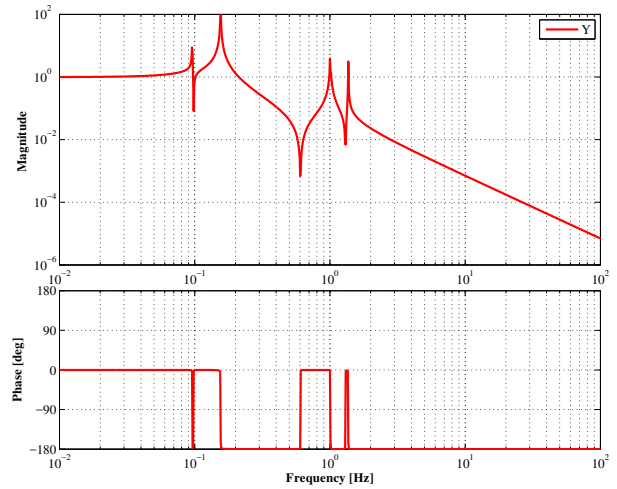
Figure 6.23: IM-OSEM (Yaw)
