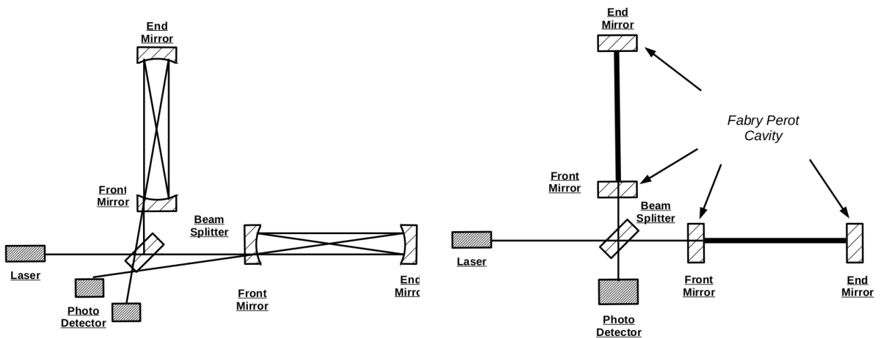
Figure 1.3: Optical configuration of a delay-line Michelson interferometer ( left ) and a Fabry-Perot Michelson interferometer ( right ).
