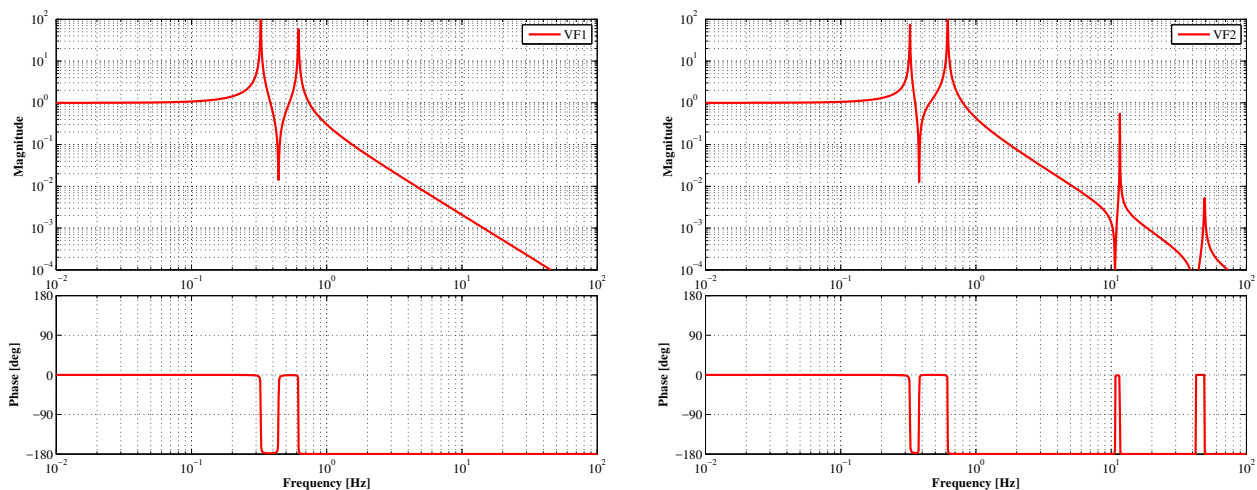
Figure 6.11: Diagonal transfer functions of GAS-LVDTs.
