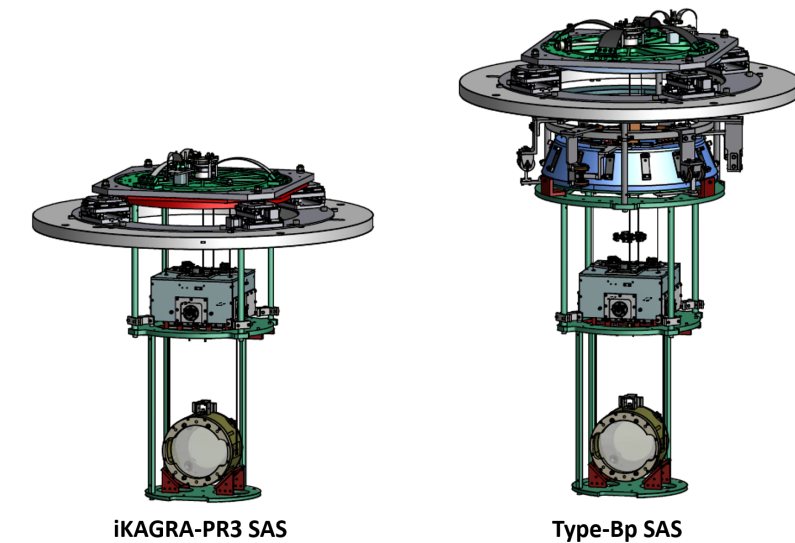
Figure 6.1: Mechanical overview of the iKAGRA-PR3 SAS ( left ) and the type-Bp SAS ( right ). In the type-Bp SAS, one GAS filter and a recoil mass for the bottom GAS filter are added into the iKAGRA-PR3 SAS.
