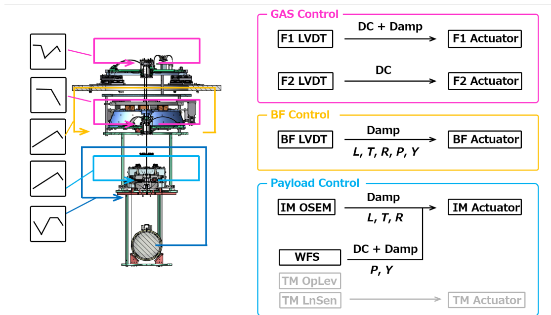
Figure 6.44: Control diagrams in observation phase with controls by IM-OSEMs.
