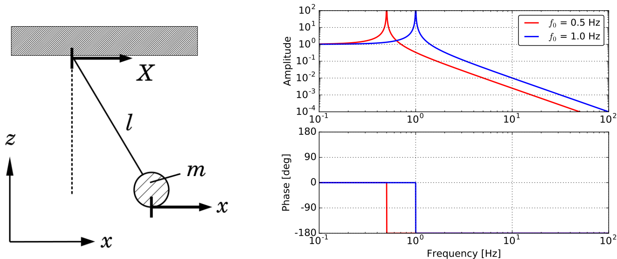
Figure 2.2: A pendulum system considered as a mechanical oscillator ( left ) and its transfer function x/X ( right ) for various resonant frequencies ( f_0 = 0.5 Hz, f_0 = 1.0 Hz). If one can lower the resonant frequency of the system, the attenuation performance at high frequencies is improved.
