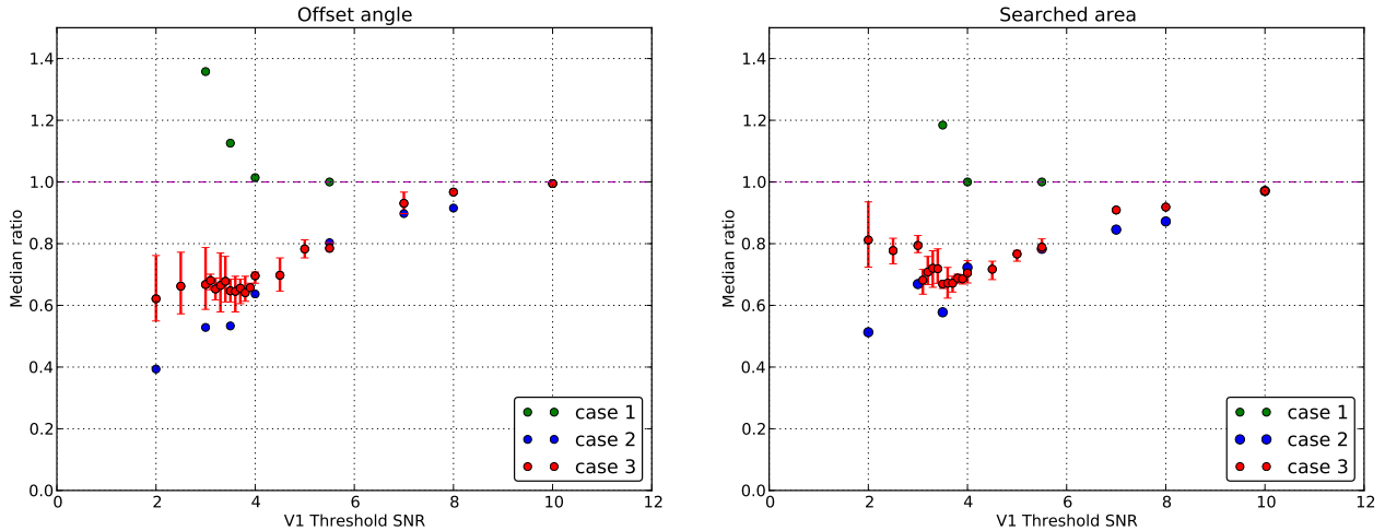
Figure 10.4: Median ratio of Offset angle ( Left ), searched area ( Right ). Both of the vertical axes are normalized with the values of the double coincidence search. In case 3 investigation, calculation is repeated for three times, using different set of random numbers.
