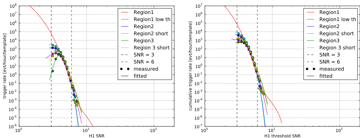
Figure 9.7: SNR distribution ( Left ), cumulative SNR distribution ( Right ). The red curve are extrapolated below SNR 6. Regions denote the template region of MBTA. The ‘low th’ shows the SNR distribution obtained by using data with lower SNR threshold. Note that this ‘Region 1 low th’ is analyzed by using 4933 templates. The ‘short’ represents the SNR distribution calculated by shorter collecting time data. The collecting time becomes longer in the order of the region 1, region 2 and the region 3. The cumulative distribution of the ‘region 1 low th’ saturates relatively at lower trigger rate. This is because there might a lot of triggers in its collecting time and miss to count large number of the triggers, compared to the other analysis except for the ‘region 3’ in the plot.
