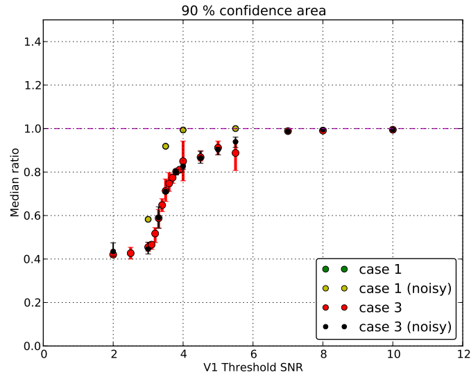
Figure 10.9: 90 % confidence area with HLV hierarchical search, when the V1 detector generates a lot of background triggers. The vertical axis is normalized with the value obtained in HL double search.
