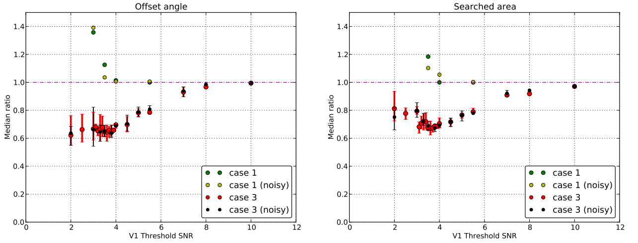
Figure 10.8: Offset angle ( Left ) and searched area ( Right ), when the V1 detector generates a lot of background triggers. In case 3 investigation, calculation is repeated for three times, using different set of random numbers.
