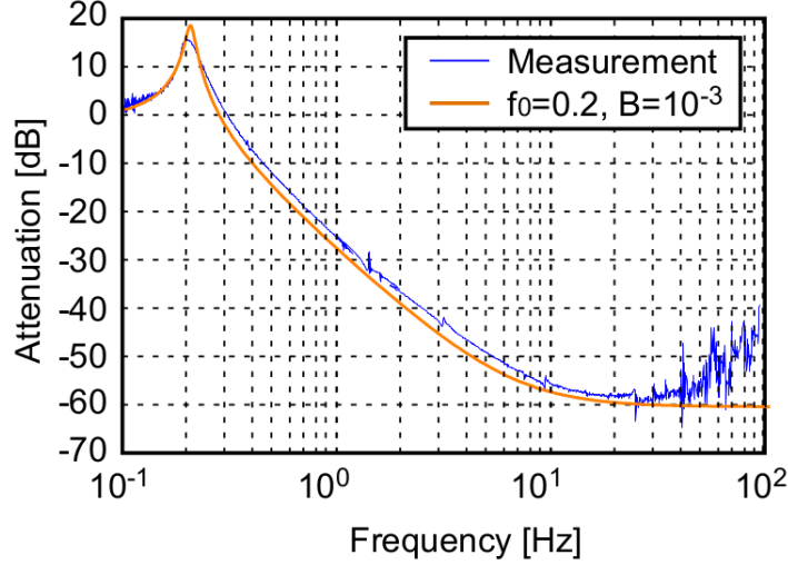
Figure 2.12: Attenuation performance of the GAS filter without the magic wand [27].
