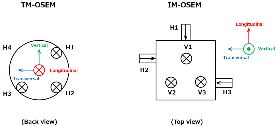
Figure 5.13: Positions of the OSEMs implemented into the payload in iKAGRA-PR3 SAS.
