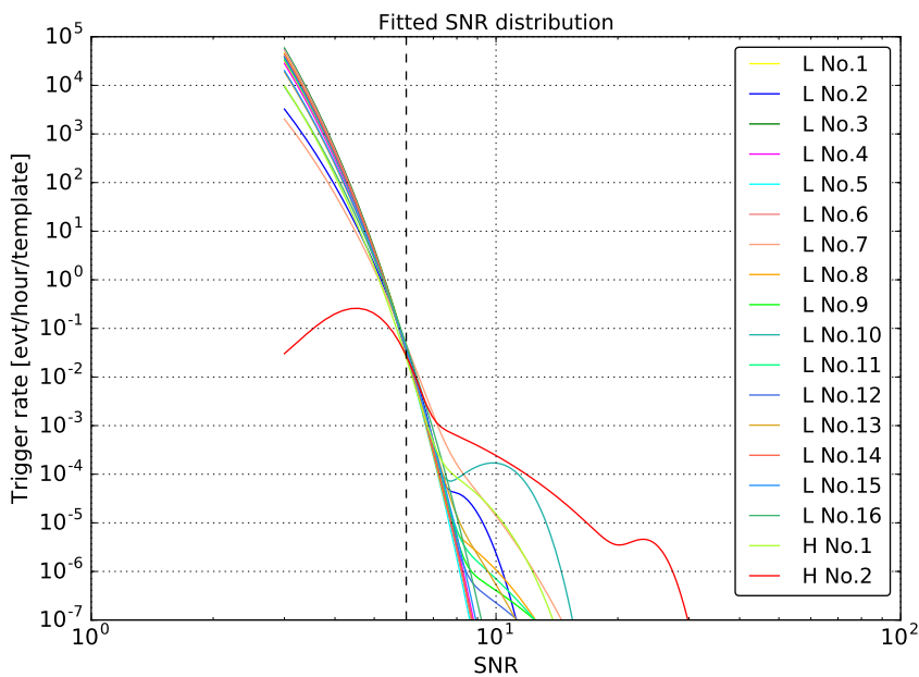
Figure 9.5: Fitted background SNR distribution at H1 and L1 detector in O1 run.
