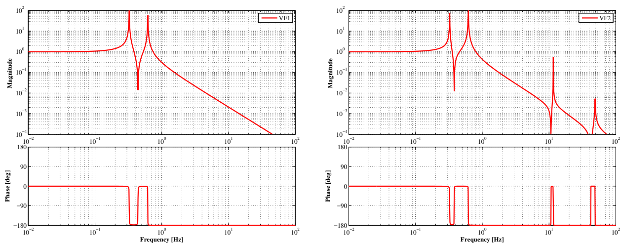
Figure 6.11: Diagonal transfer function measured by GAS-LVDTs.
