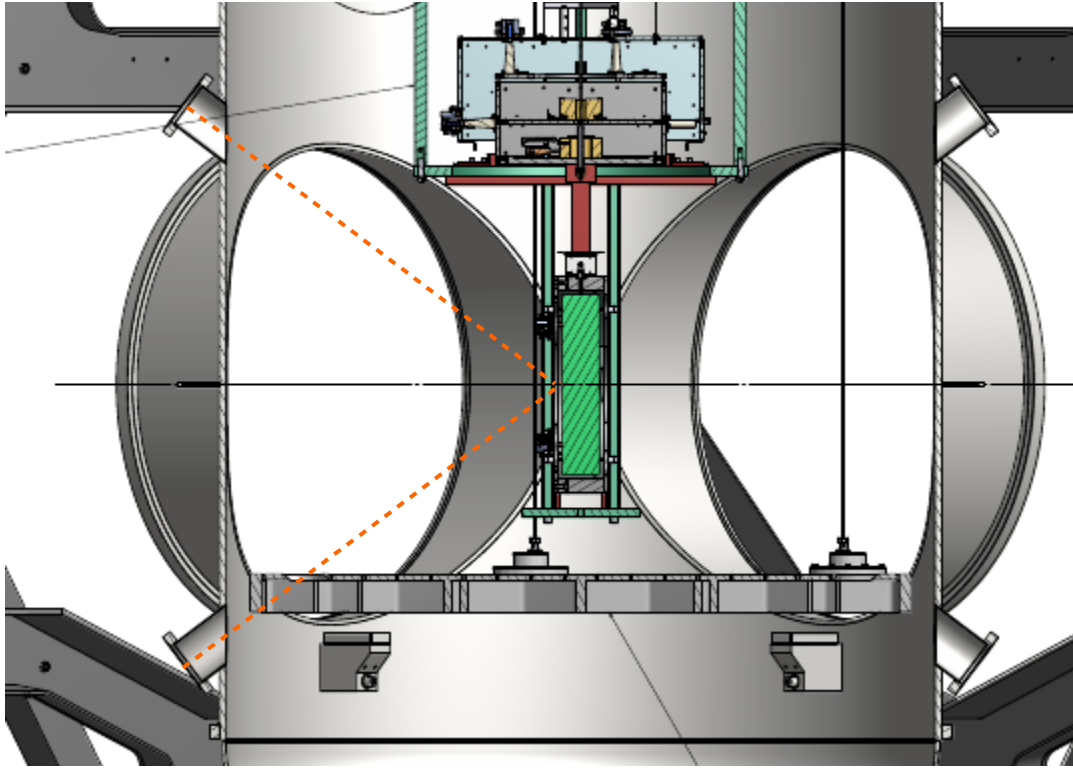
Figure 6: Drawing of the beam-splitter chamber and the path of the OpLev beam (Orange). The total length of this path is 2 \times 988.8 mm.
