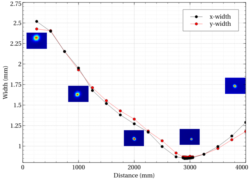
Figure 4: Development of the beam profile of the used collimator in two dimensions. The small pictures are photographs of the actual profile. The width means the actual diameter of the beam.
