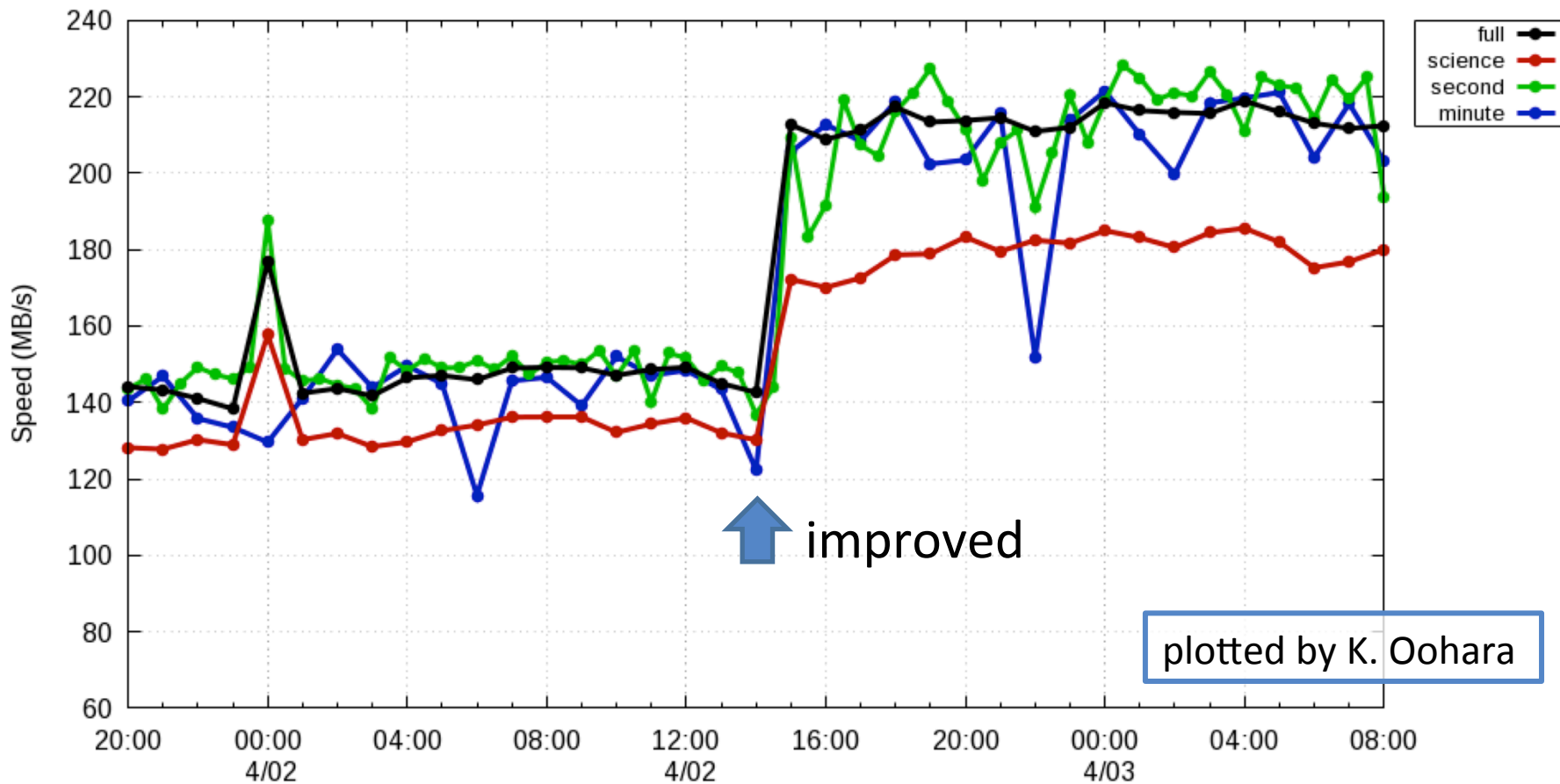
Speed of Transfer: Kamioka(underground) \Rightarrow Kamioka(surface)
