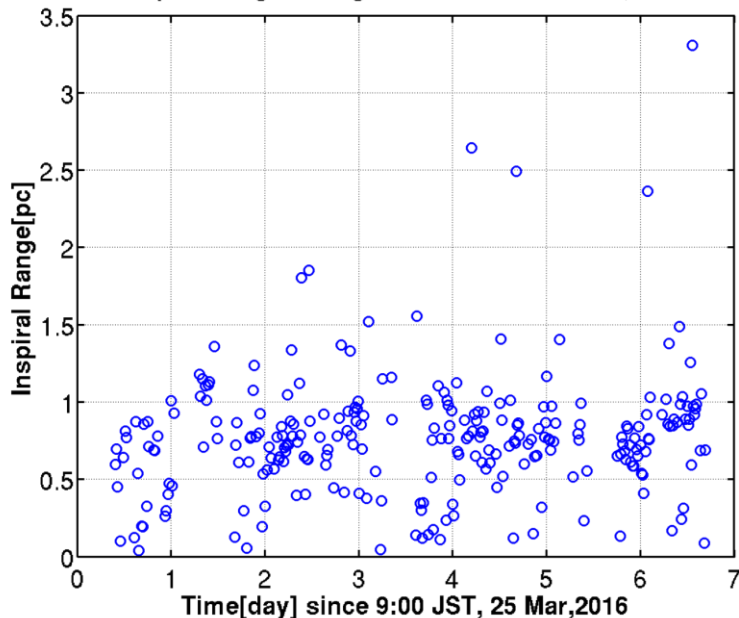
inspiral range during iKAGRA run in March, 2016
