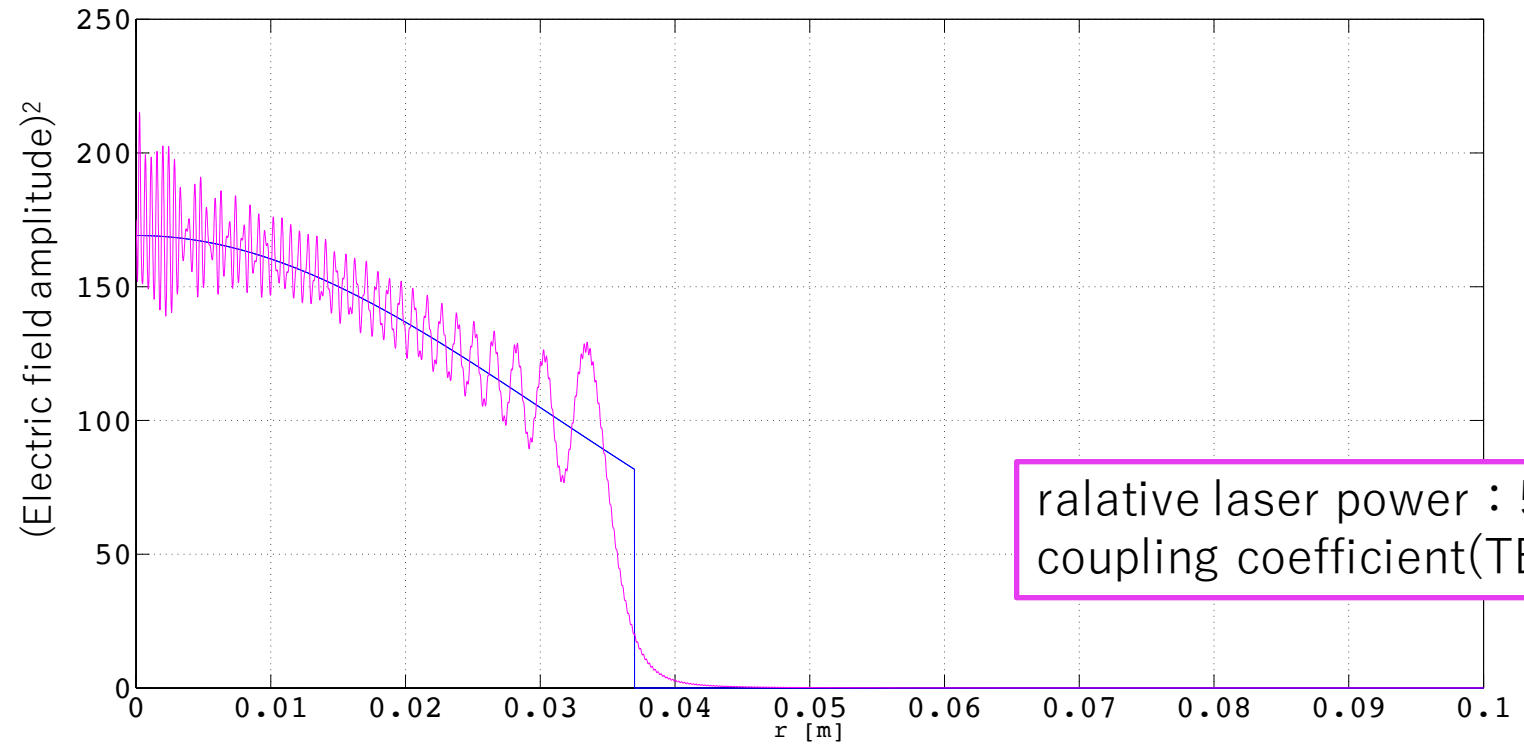
beam profile
