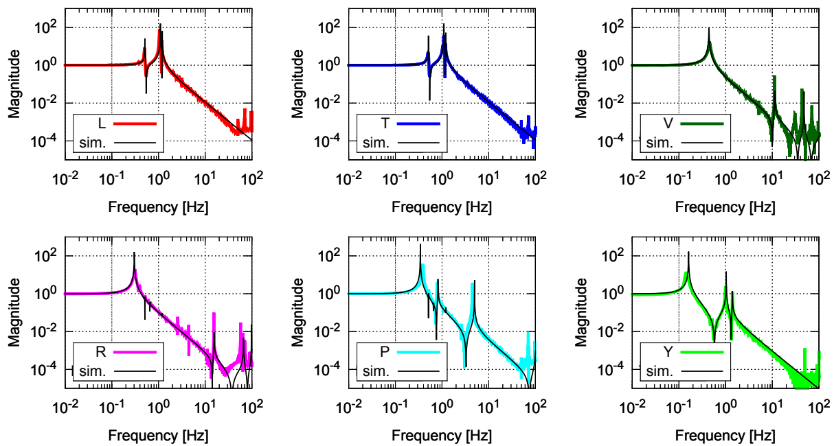
Figure 6.37: Comparison of diagonal transfer functions measured by IM-OSEMs (shown in colored lines) and prediction from the rigid-body model simulation (shown in black lines).
