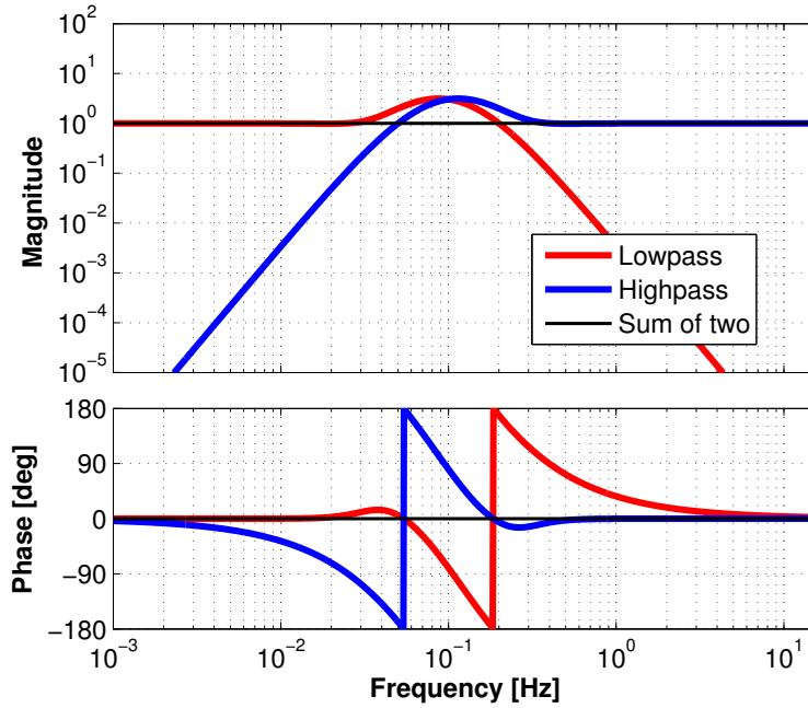
Figure 5.6: Bode plots of the blinding filters with the crossover frequency of 0.1 Hz.
