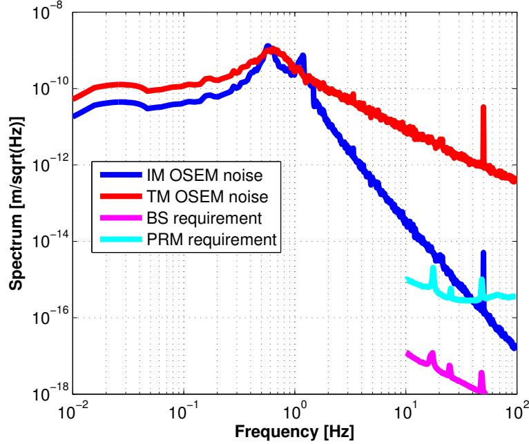
Figure 5.15: Sensor noise couplings of the payload damping controls in the type-B SAS.
