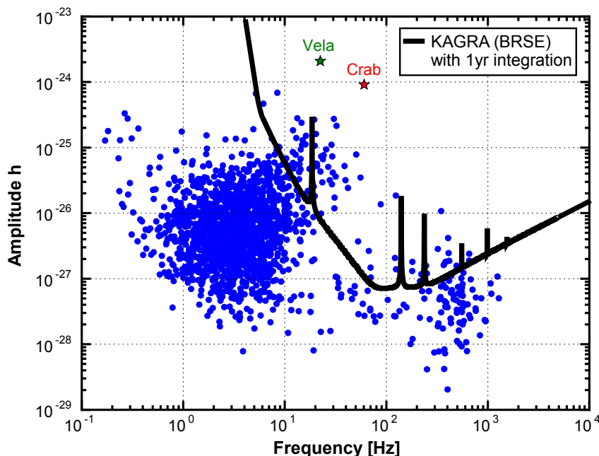
Figure 1.11: The maximum gravitational wave amplitude of the know spinning pulsars [36], overlaid with the KAGRA sensitivity with 1 year integration.
