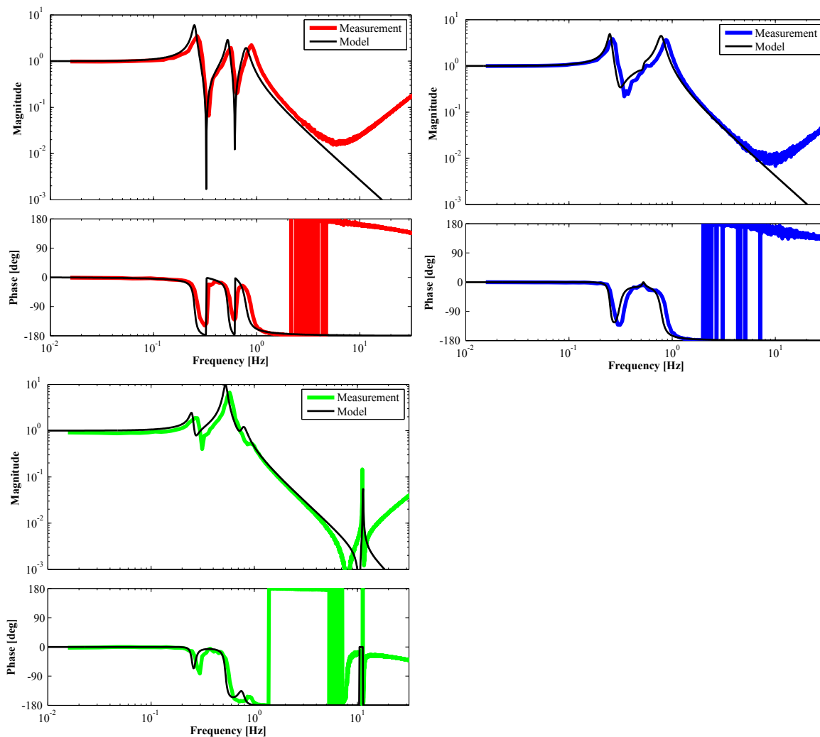
Figure 7.6: Comparison of measured transfer functions about GAS filters and prediction from simulation.
