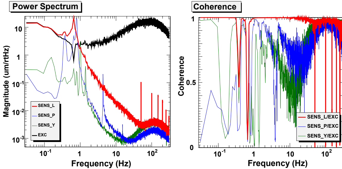
Figure 7.2: (Left) Spectra of the excitation signal in the TM longitudinal DoF and measured displacement signals. (Right) Coherence between the excitation signal and sensor signals.
