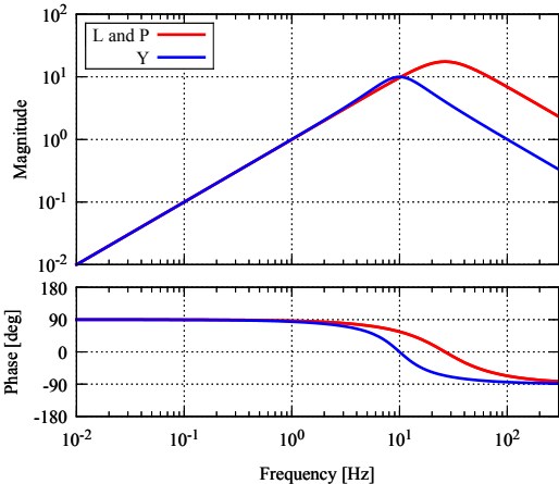
Figure 7.8: TM control servo filters.
