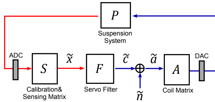
Figure 7.12: Signal flows in the open loop gain measurement.
