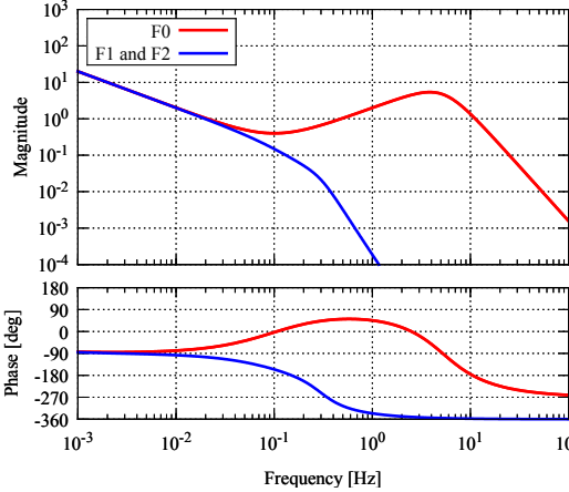
Figure 7.11: GAS control servo filters.
