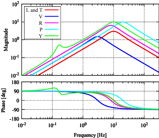
Figure 7.9: IM control servo filters.
