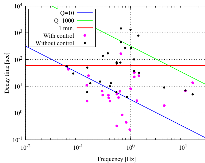
Figure 7.13: Decay time versus resonant frequency plot.
