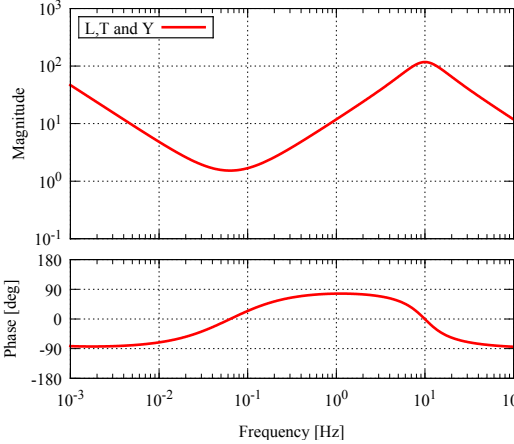
Figure 7.10: F0 control servo filters.
