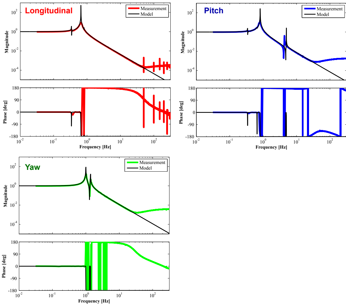
Figure 7.3: Comparison of measured transfer functions about TM and prediction from the rigid-body model simulation.
