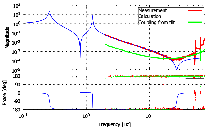
Figure 5.19: Multi-SAS 用倒立振り子の伝達関数
