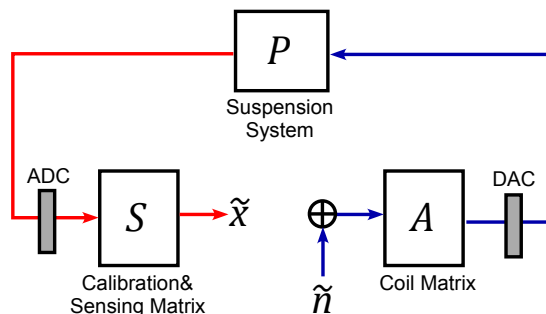
Figure 7.1: Signal flows in the transfer function measurement.
