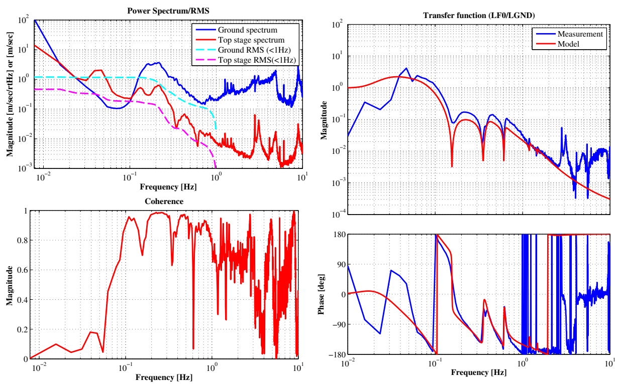
Figure 7.15: IP transfer function measurement with control
