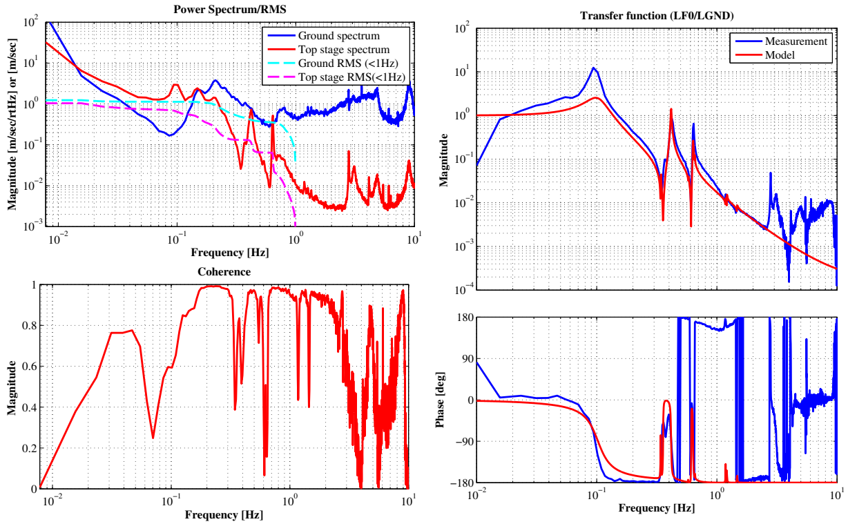
Figure 7.14: IP transfer function measurement without control
