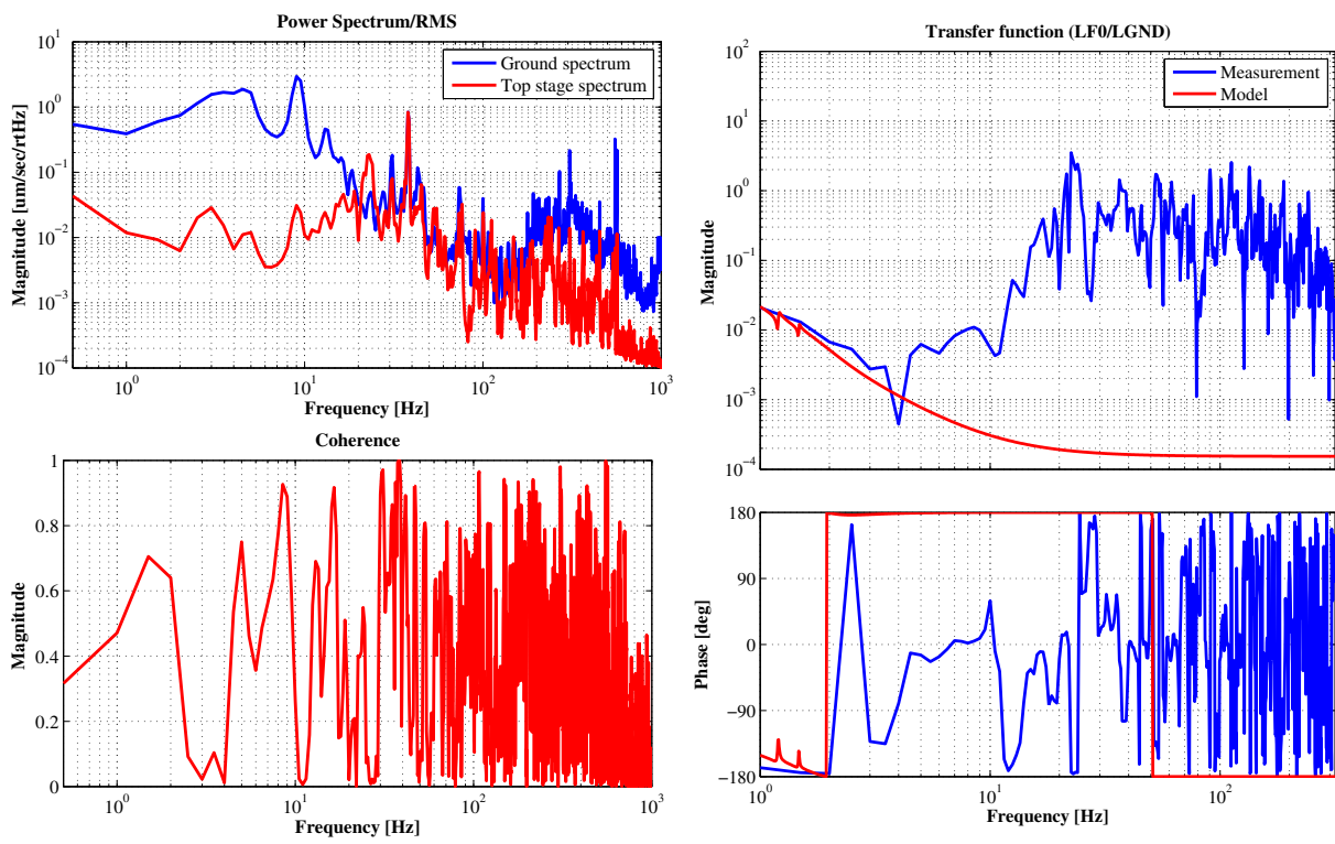
Figure 7.16: IP transfer function measurement high frequency
