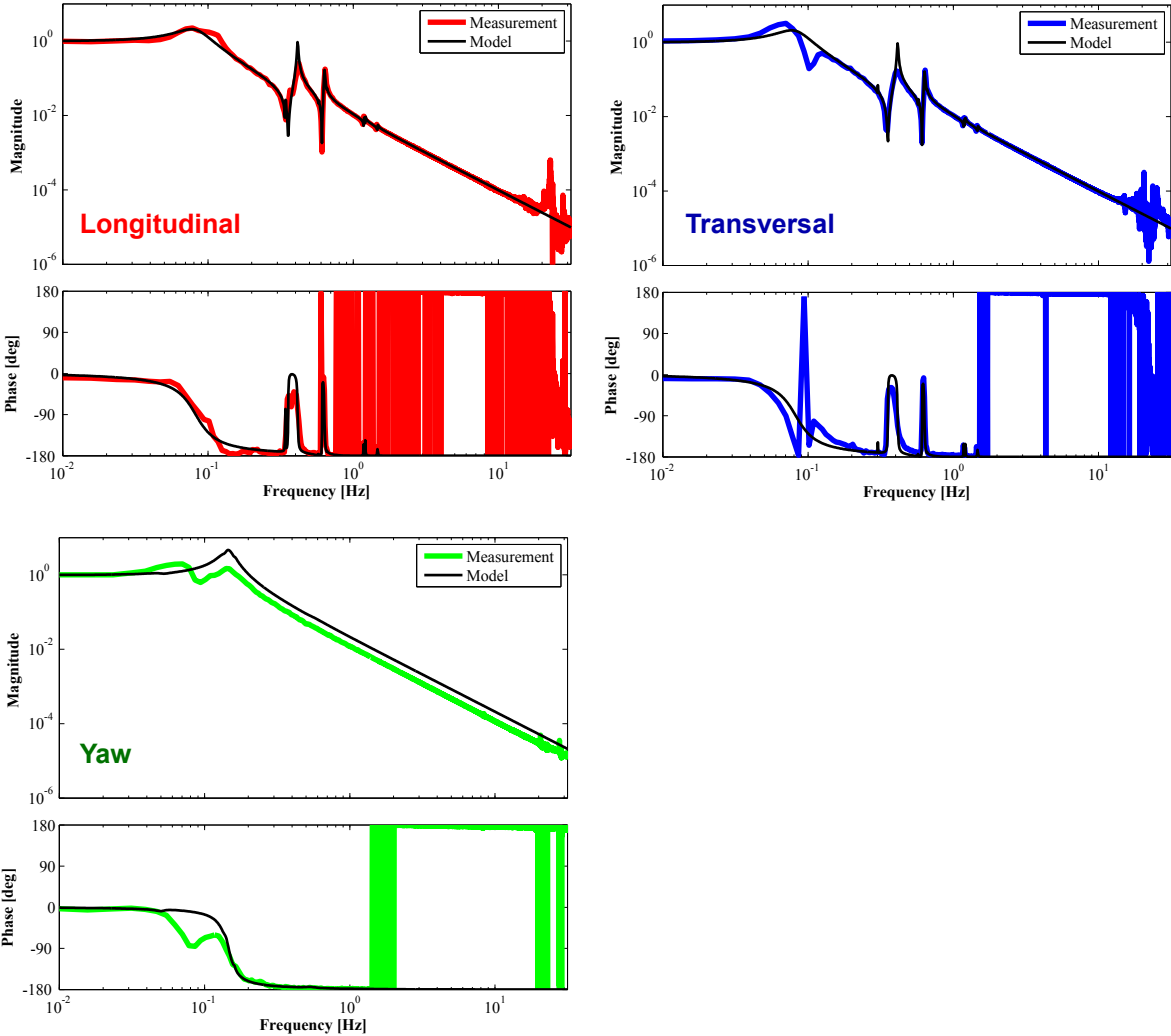
Figure 7.5: Comparison of measured transfer functions about F0 and prediction from simulation. The simulation does not take into account any asymmetry in the IP stiffness.
