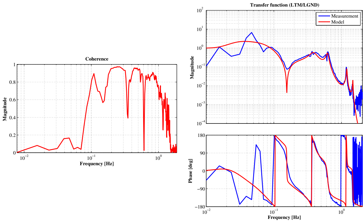
Figure 7.17: Transfer function from ground to TM.
