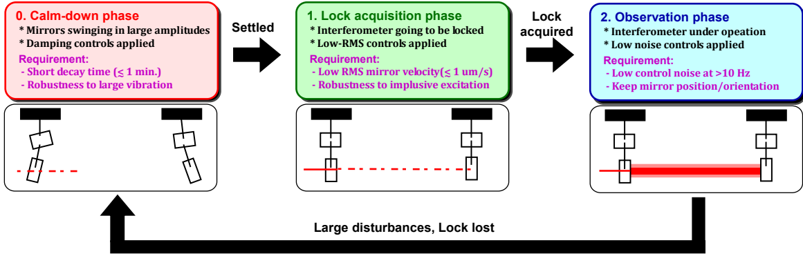
Figure 4.1: Digram of active control phases and the requirements in each phase.
