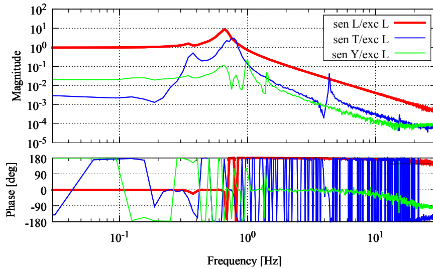
Figure 7.7: Measured transfer functions from the TM-RM longitudinal actuator to the displacements including the coupling with other DoFs.
