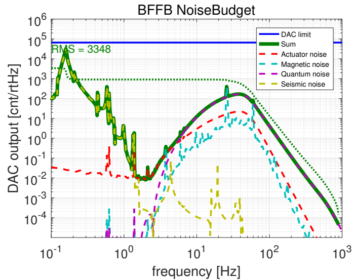
Figure 31: Spectra of feedback signals for the ETMBF.
