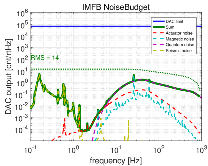
Figure 33: Spectra of feedback signals for the ETMIM.
