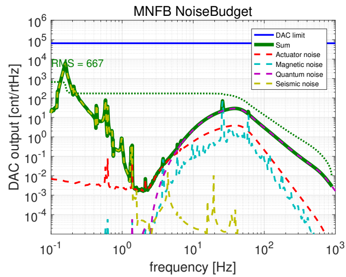
Figure 32: Spectra of feedback signals for the ETMMN.
