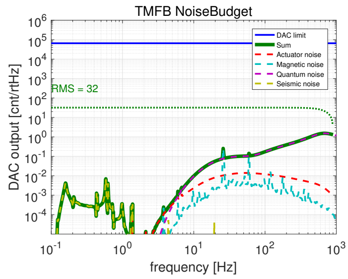
Figure 34: Spectra of feedback signals for the ETMTM.
