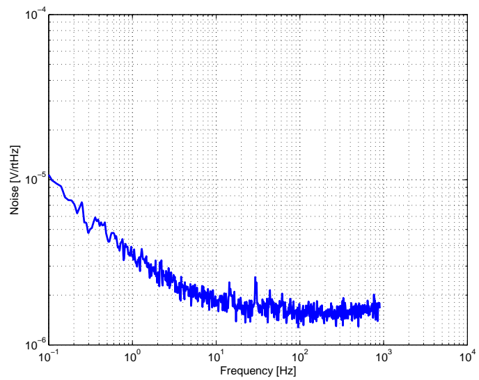
Figure 8: DAC noise.
