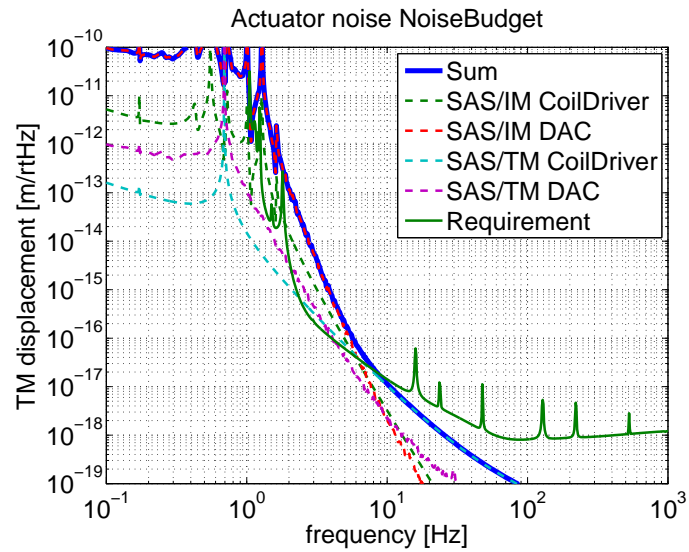
Figure 11: Actuator noise budget for BS.
