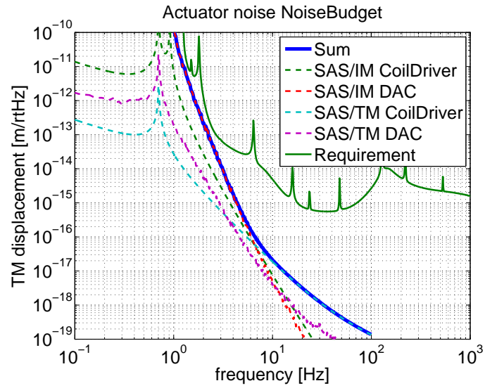
Figure 19: Actuator noise budget for PRM.
