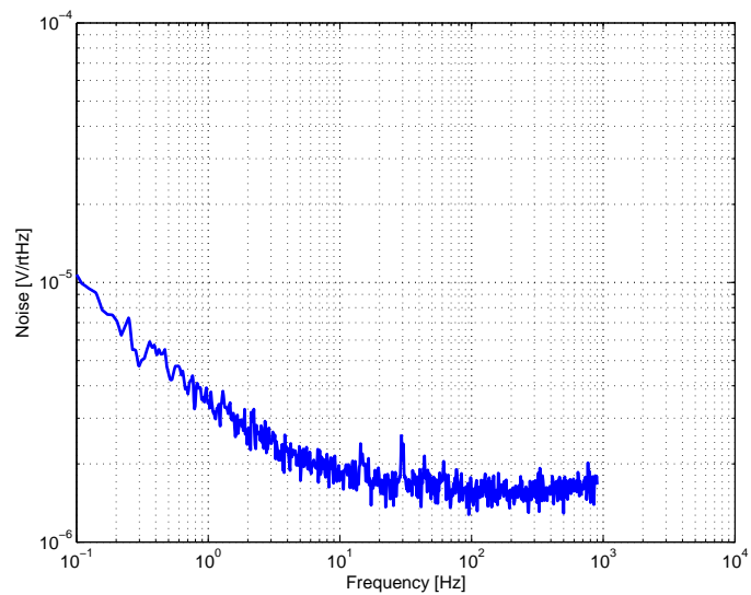
Figure 8: DAC noise.
