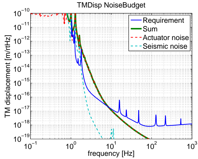
Figure 10: Displacment noise budget for BS.
