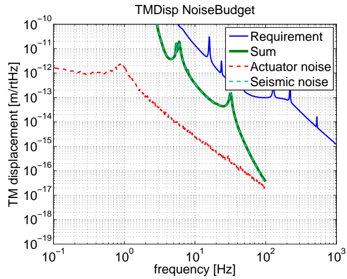
Figure 22: Displacment noise budget for IMC.
