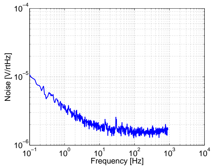
Figure 8: DAC noise.
