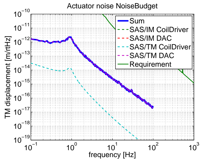
Figure 23: Actuator noise budget for IMC.
