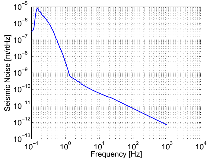
Figure 4: Kamioka seismic noise.
