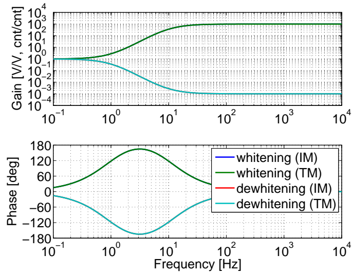
Figure 6: Whitening and dewhitening filters for IM and TM.
