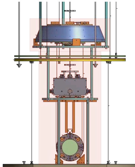
Figure 4: Payload, composed by the bottom filter, the intermediate mass and its recoil mass, the mirror and its recoil mass, and the lower section of the safety structure.
