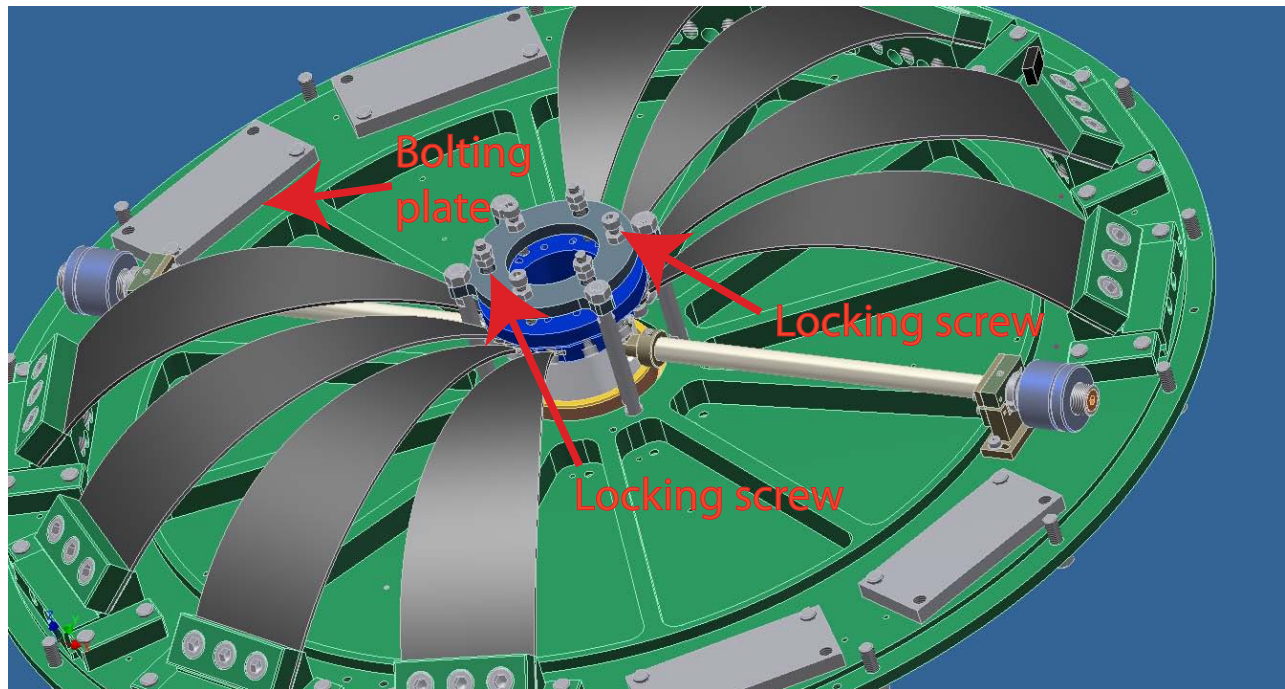
Figure 11: The three locking screws and nuts lock the vertical movement of the GAS springs. Bolting plates have been added in the empty slots of missing blades to provide threaded holes to lock the filter to its safety structure as illustrated in figure 12
