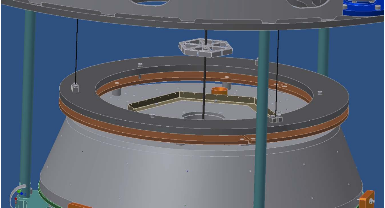
Figure13: Three bolts lock the magnetic damper ring to its copper ring on the top of the standard filter.
