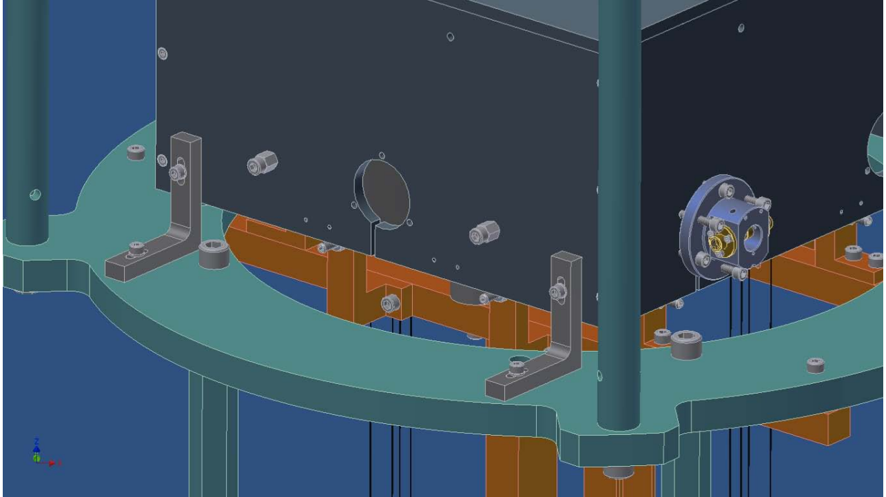
Figure19: Four brackets lock the transversal movement of the intermediate recoil mass. Note: slots are foreseen in the brackets because the intermediate mass and its recoil mass are first interlocked by tightening their mutual motion range limiting screws. The brackets are tightened down last.
