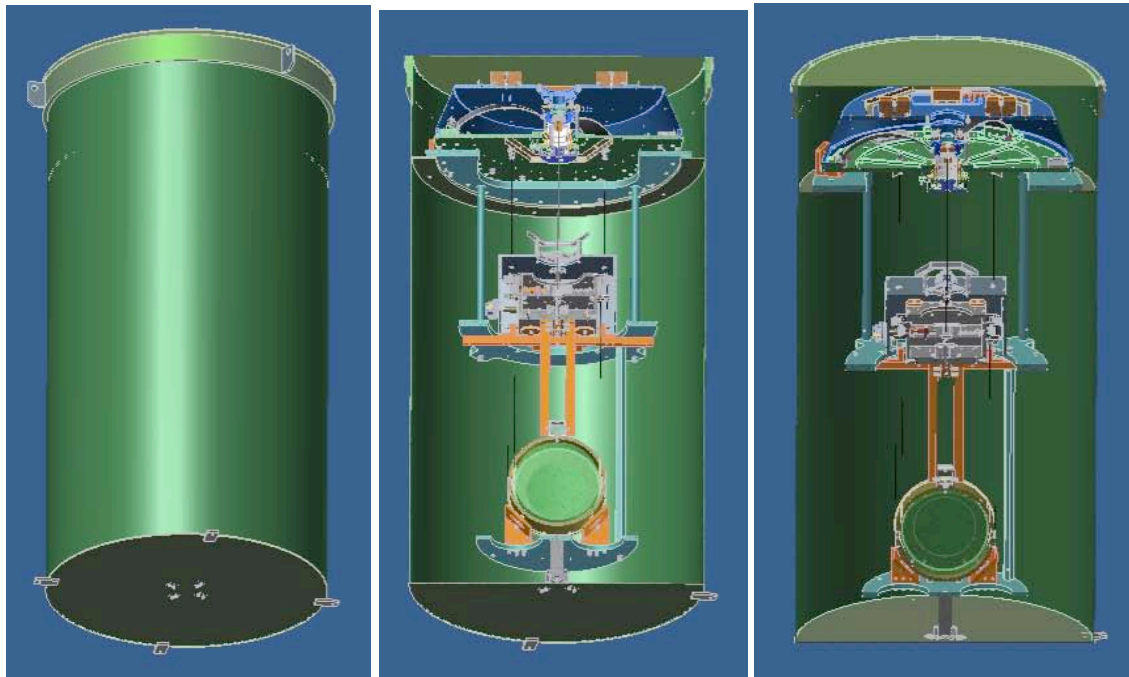
Figure 16: The transport tank for the payload is much smaller. The bottom plate of the tank is provided with bolting lips to attach the tank to a transport pallet. The payload locked into its safety structure is bolted from above onto a circular shelf.
