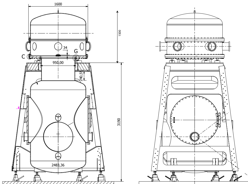
Figure 22: dimensions of the Type-B SAS towers.
