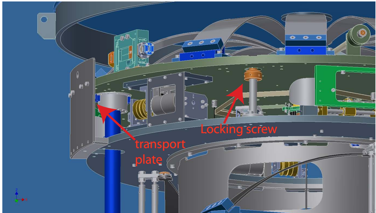
Figure 10 The orange screw-head are engaged to lock the horizontal movement of the IP. Then the transport plates are mounted to lock the Inverted pendulum to the base structure of the pre-isolator.
