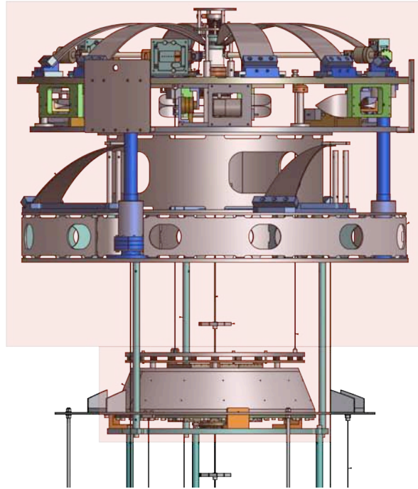
Figure 3: Seismic attenuation, composed of the pre-isolator, the standard filter, the Eddy current damper and the top part of the safety structure.
