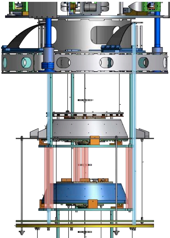
Figure 5: Components to be removed to section the seismic isolation from the payload. Shaded in pink are the mirror suspension wire and the four tie rods connecting the upper and lower section of the earthquake safety structure. Shaded in light blue are the three suspension wires of the optical bench intermediate mass.
