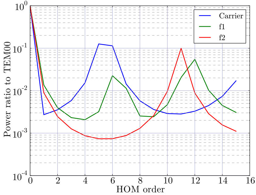
Figure 2.17: HOM power ratio in the PRC.
