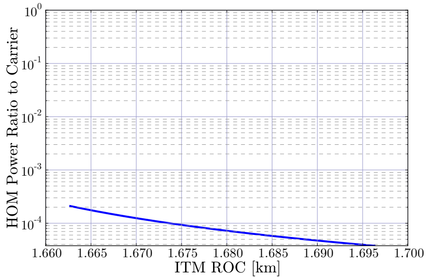
Figure 2.4: The maximum HOM power ratio in the AC as a function of ITM ROC error for the negative g -factors. The ROC is swept by \pm 1\% around the nominal value.
