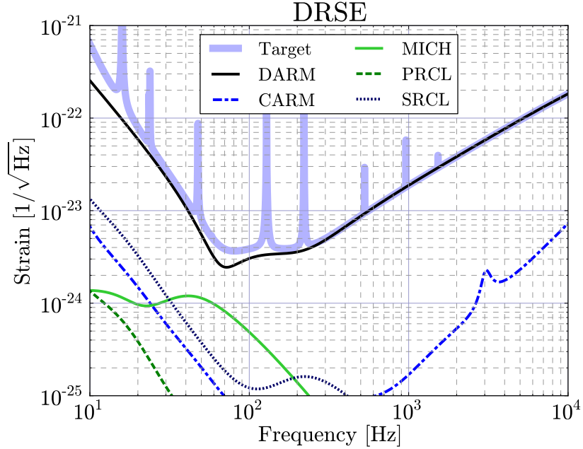
Figure 3.6: Loop Noise Coupling with Feed Forward: DRSE
