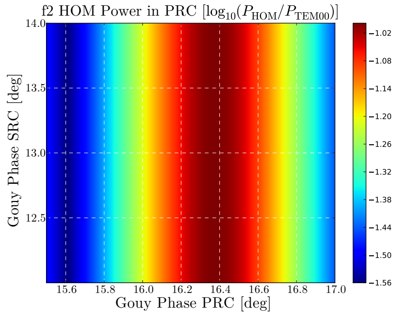
Figure 2.24: The maximum HOM power ratio of the f2 SB in the PRC, zoomed.
