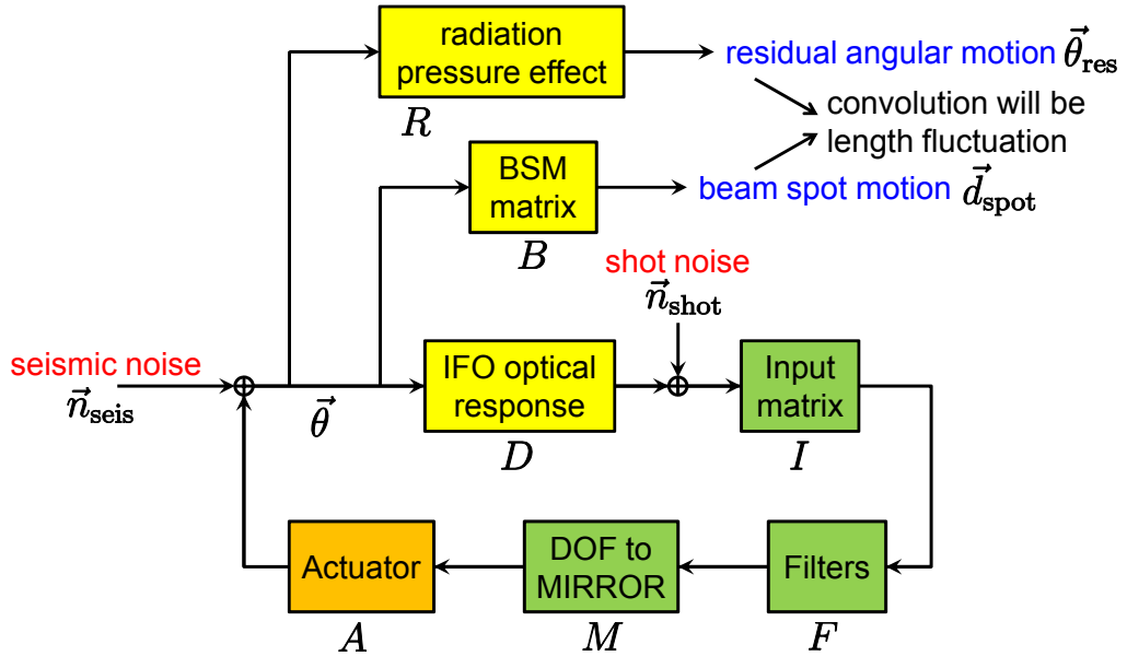
Figure 5.3: Structure of the ASC model.
