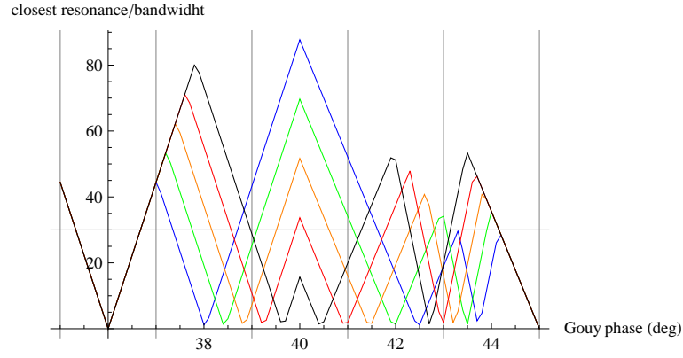
Figure 2.30: Frequency margin to the closest resonance of any higher order modes up to the 8th mode. The black, red, orange, green and blue curves correspond to the OMC length of 90, 80, 70, 60, and 50 cm, respectively. The horizontal line at the center indicates the suppression rate of 45 dB.
