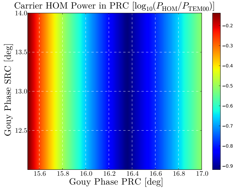
Figure 2.22: The maximum HOM power ratio of the carrier in the PRC, zoomed.
