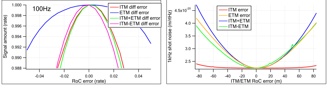
Figure 2.29: Left : Signal loss due to the differential RoC errors of the test masses, and Right : Shot noise increase due to the junk light caused by the differential RoC errors of the test masses.
