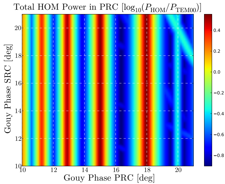
Figure 2.21: The maximum HOM power ratio of the total field in the PRC.
