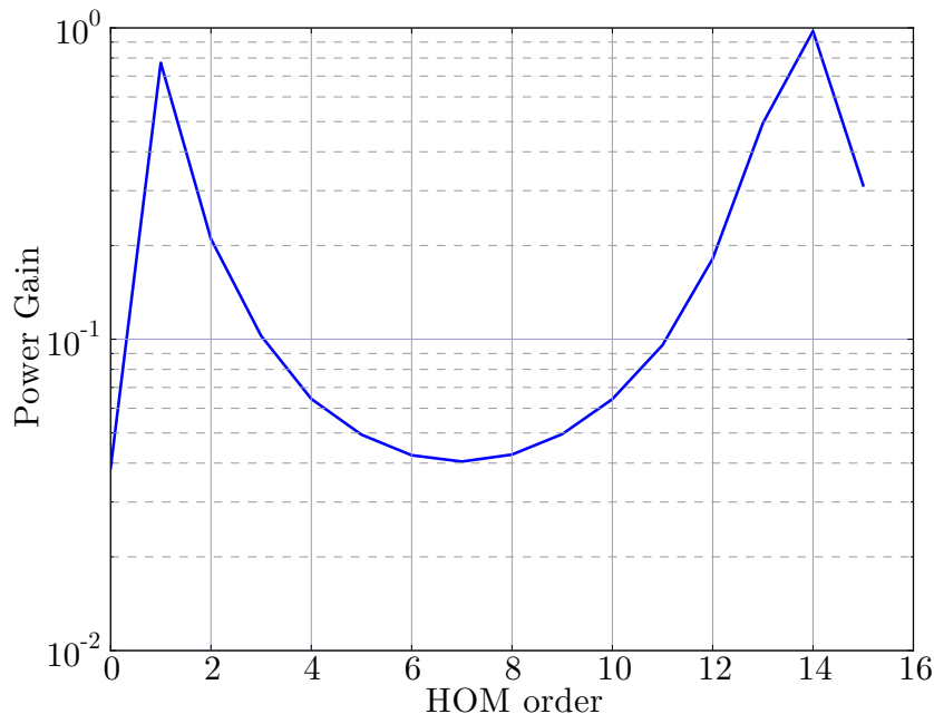
Figure 2.27: The SRC HOM power build up gain.
