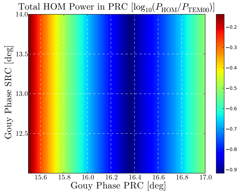
Figure 2.25: The maximum HOM power ratio of the total field in the PRC, zoomed.
