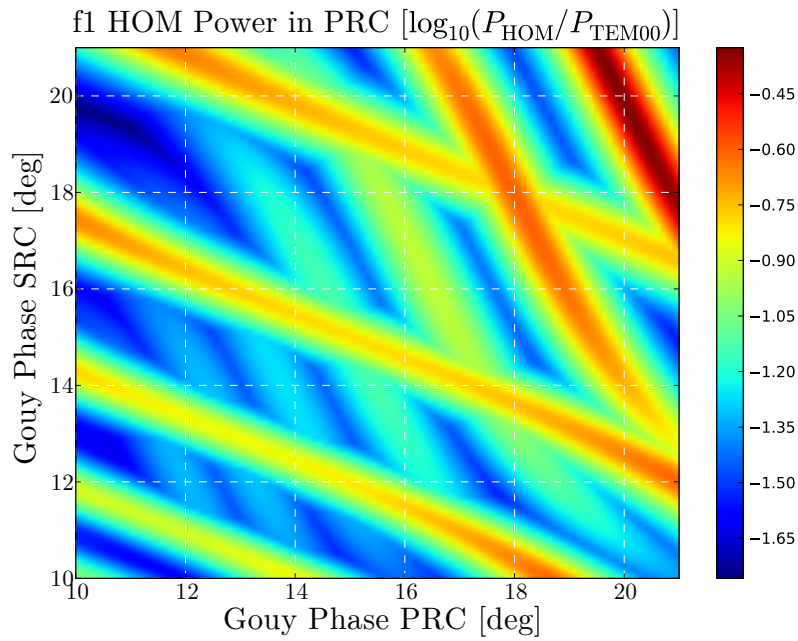
Figure 2.19: The maximum HOM power ratio of the f1 SB in the PRC.
