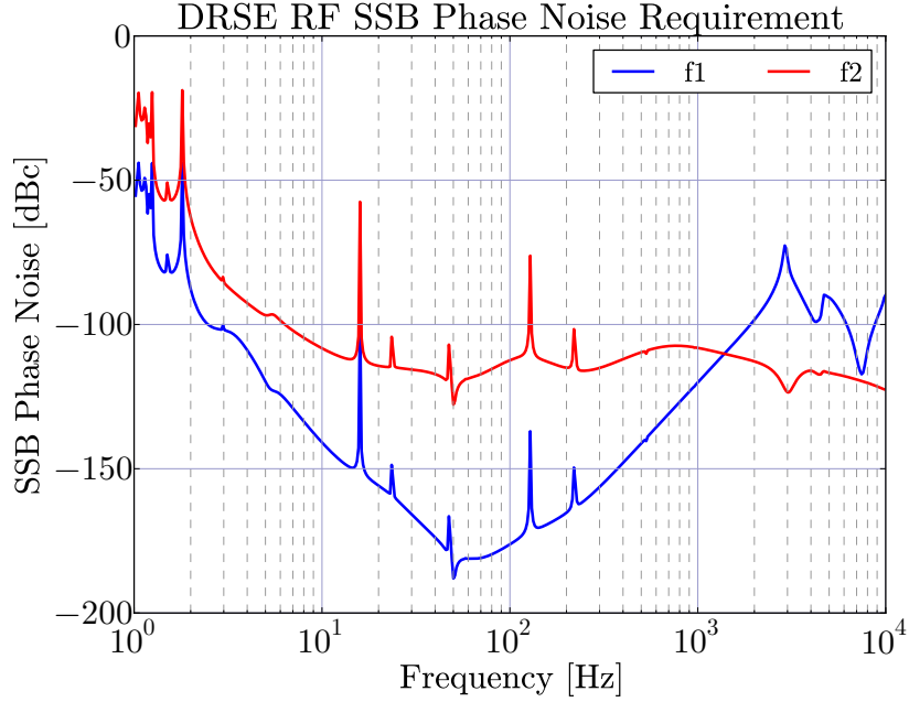
Figure 4.11: SSB Phase noise requirements: DRSE
