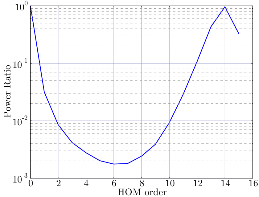
Figure 2.26: The SRC HOM power build up compared to the completely degenerated SRC.
