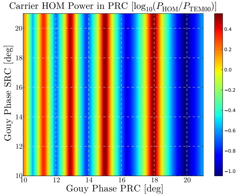
Figure 2.18: The maximum HOM power ratio of the carrier in the PRC.
