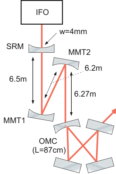
Figure 2.28: Output mode-cleaner system.
