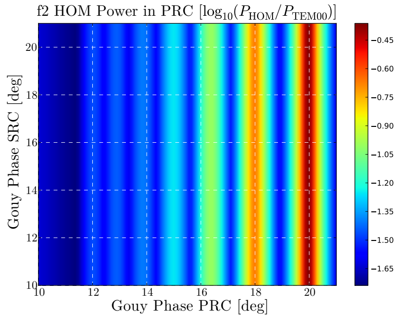
Figure 2.20: The maximum HOM power ratio of the f2 SB in the PRC.
