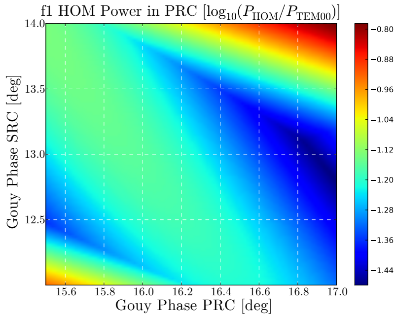
Figure 2.23: The maximum HOM power ratio of the f1 SB in the PRC, zoomed.
