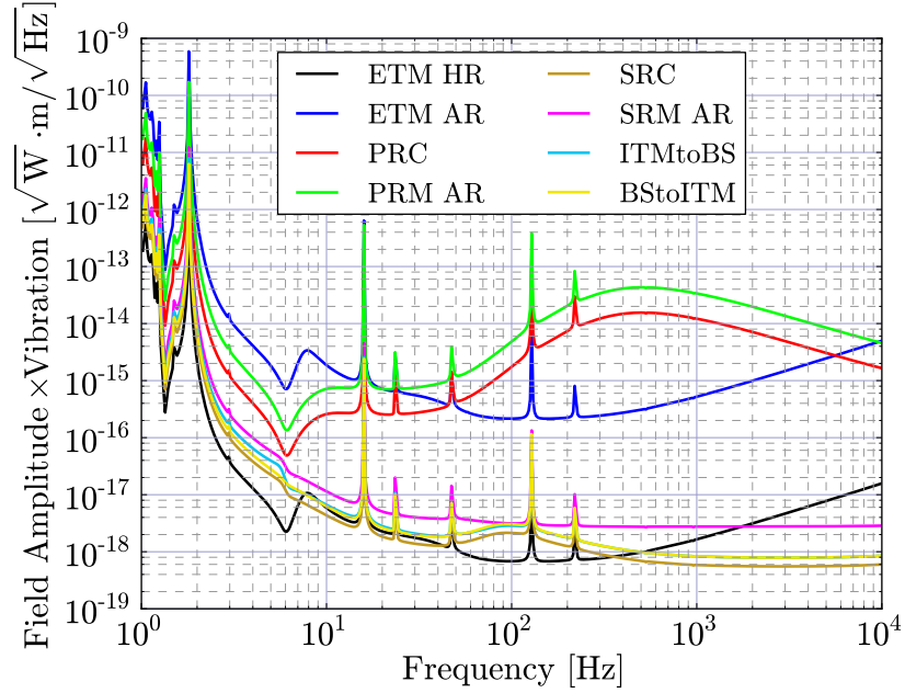
Figure 4.14: Scattered light requirements: BRSE
