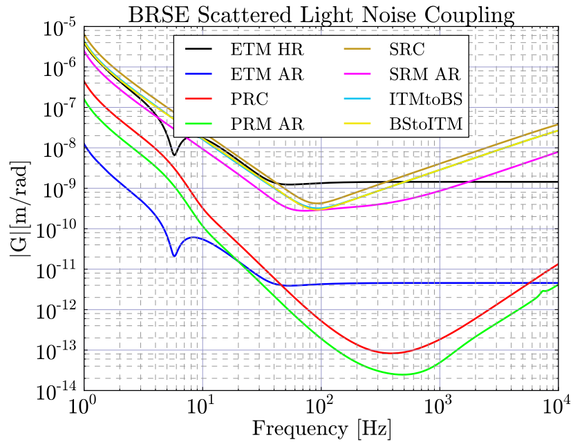
Figure 4.16: Coupling coefficients of scattered light: BRSE
