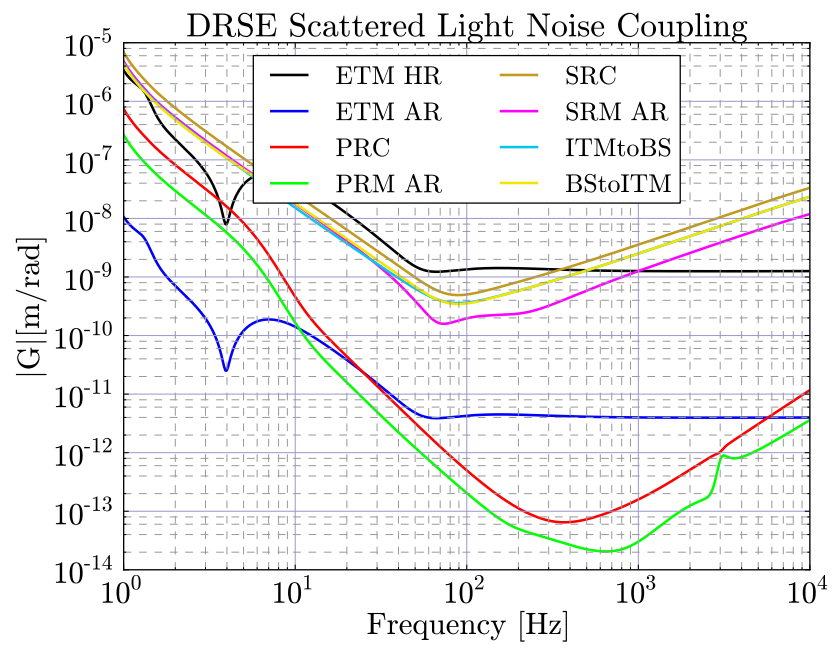
Figure 4.17: Coupling coefficients of scattered light: DRSE
