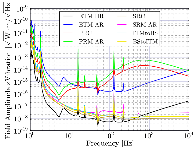
Figure 4.15: Scattered light requirements: DRSE
