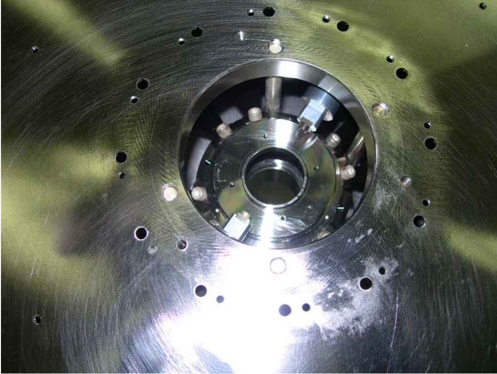
After mounting the magic wands, the LVDT primary and the actuation coil are mounted on the filter.
