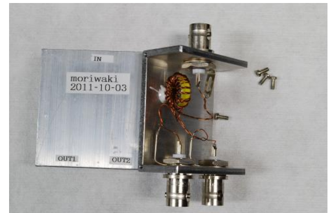
Power splitter
